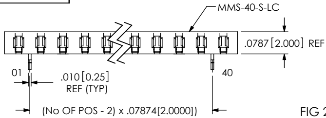
FIG 2 MMS-140-02-XXX-SH-LC SHOWN
