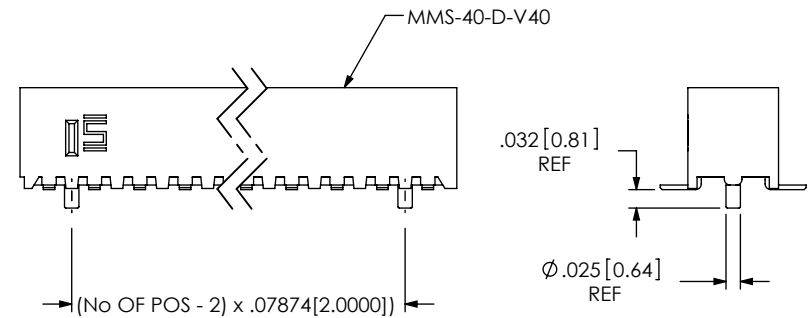
FIG 4 -A: MOLDED ALIGNMENT PIN ONLY AVAILABLE ON -DV MMS-140-02-XXX-DV-A SHOWN SAME AS FIG 1, EXCEPT AS SHOWN
