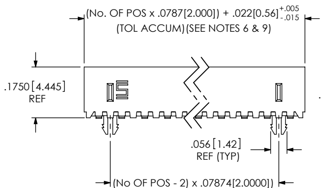
FIG 1 MMS-140-02-XXX-XV-LC SHOWN
