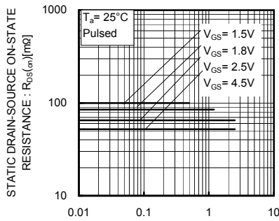
Fig.4 Static Drain-Source On-State Resistance vs. Drain Current( I )
