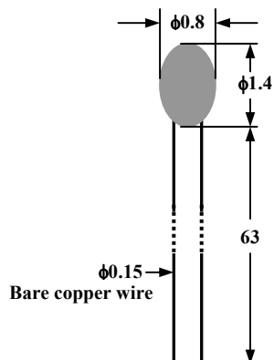
Figure 1 Side View of ATH100KR8
