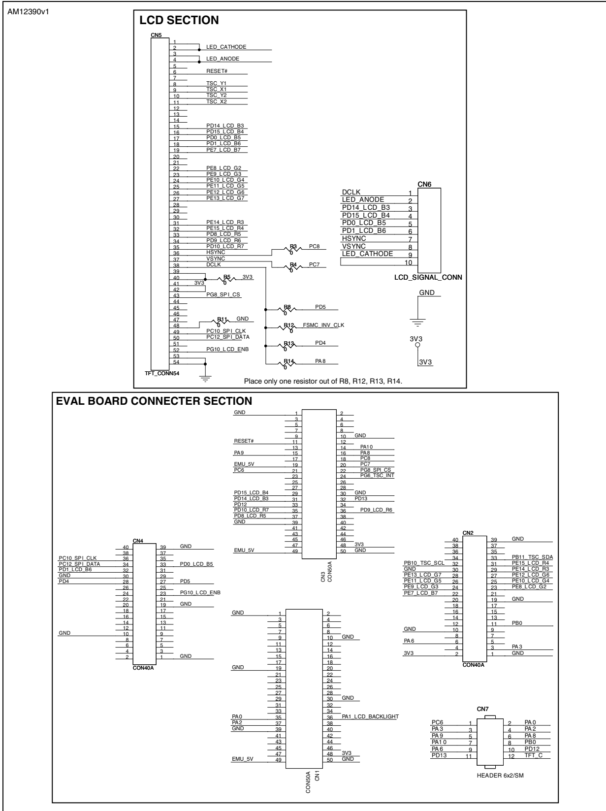
Figure 2. STEVAL-CCM004V1 schematic (part 2)
