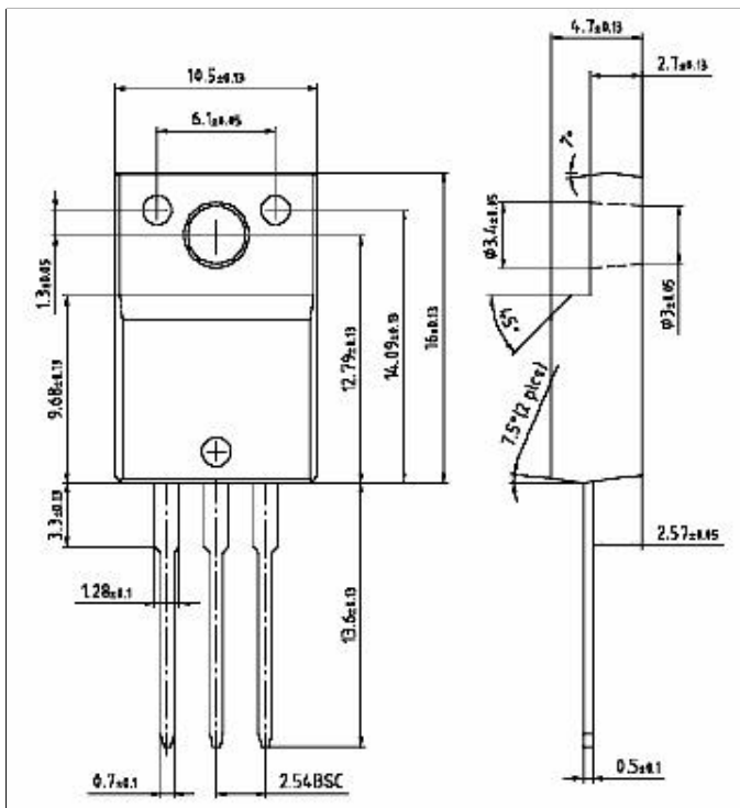
P-TO-220-3-31 (FullPAK)
