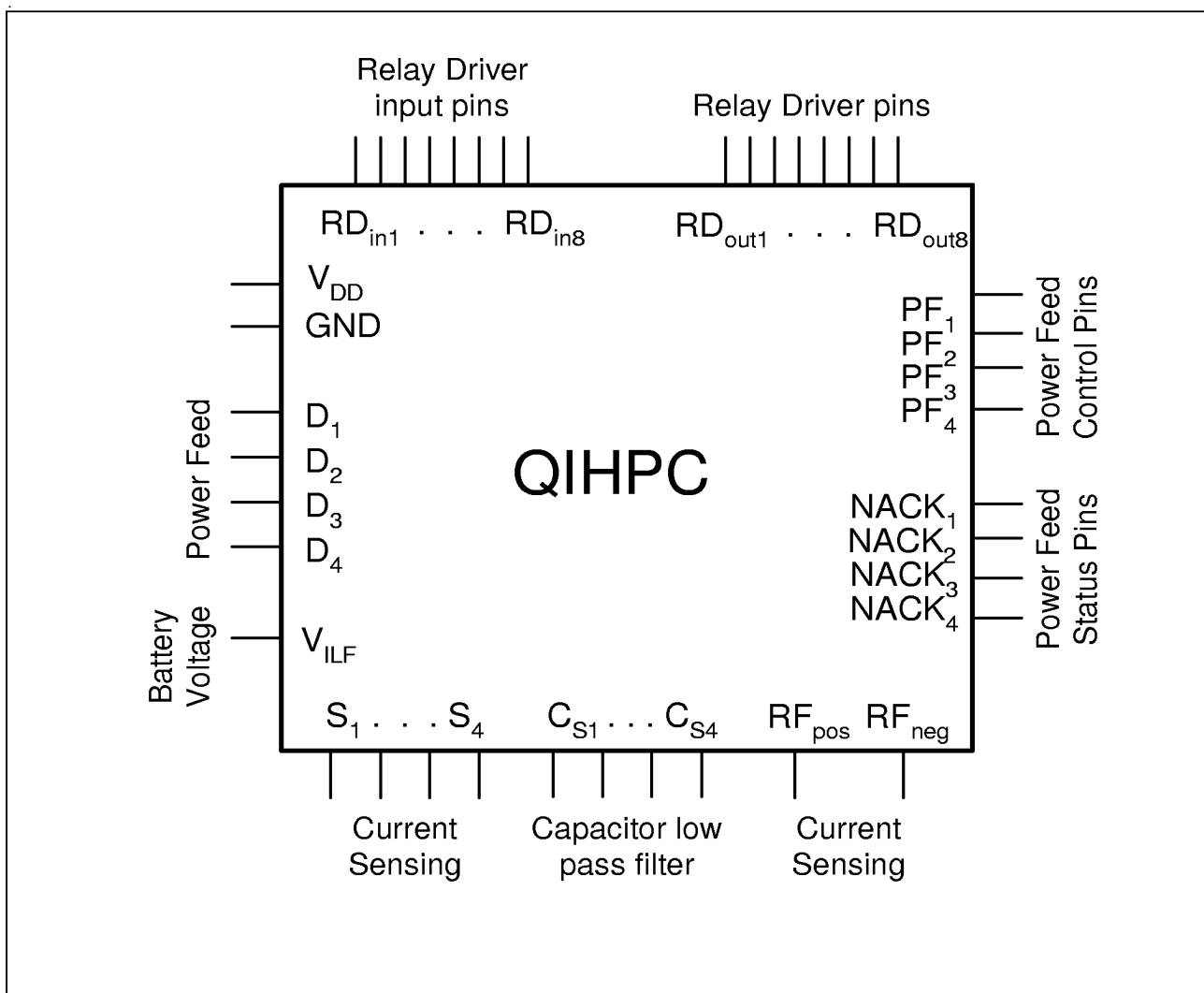
Figure 1 Logic Symbol
