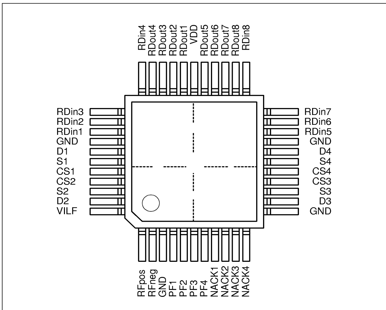
Figure 4 Pin Configuration
