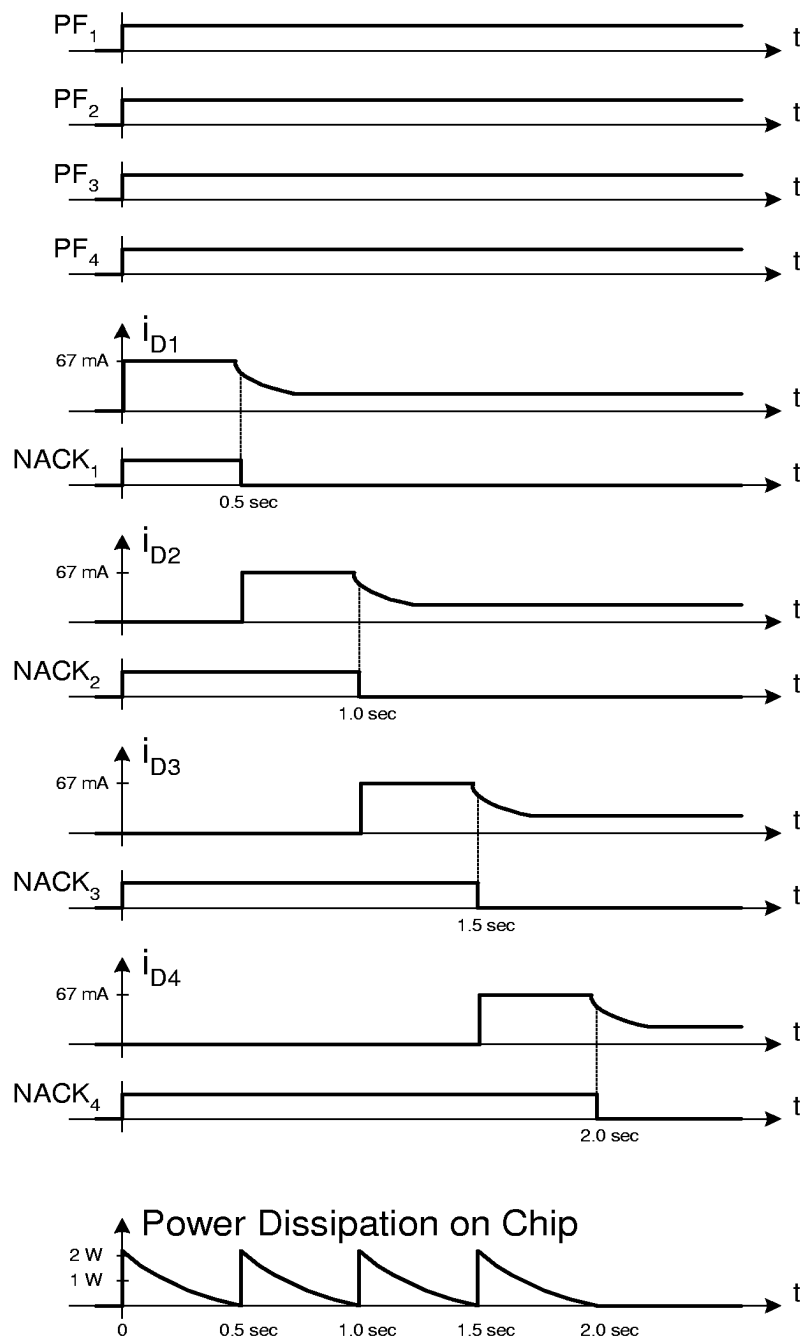
Figure 9 Simultaneous Power Up Sequence
