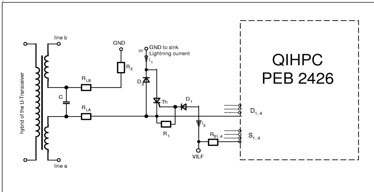
Figure 7 Proposal for a Protection Circuitry
