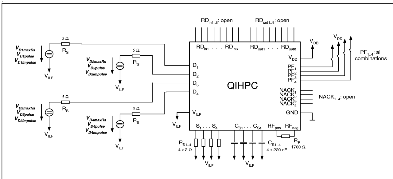
Figure 15 Test circuit for maximum DC-voltages, pulse voltages and impulse voltages on pins D_{1..4}
