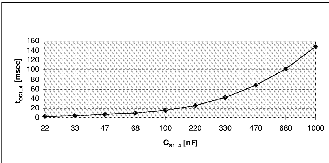
Figure 6 Delay time t_{OC} as a function of the value of C_{S1..4} (typical values)
