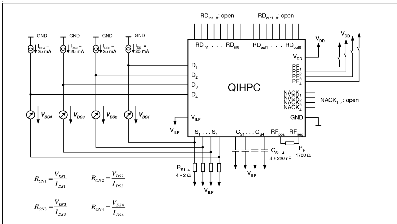
Figure 12 DMOS- R_{ON} resistance
