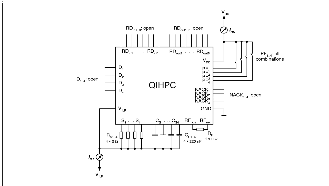
Figure 10 Supply Currents
