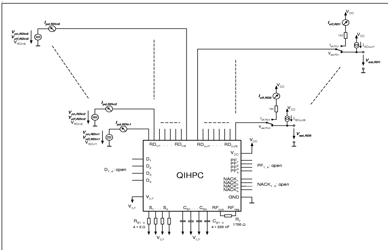
Figure 14 RD_{in1..8} , Relay Driver Inputs and RD_{out1..8} Relay Driver Outputs
