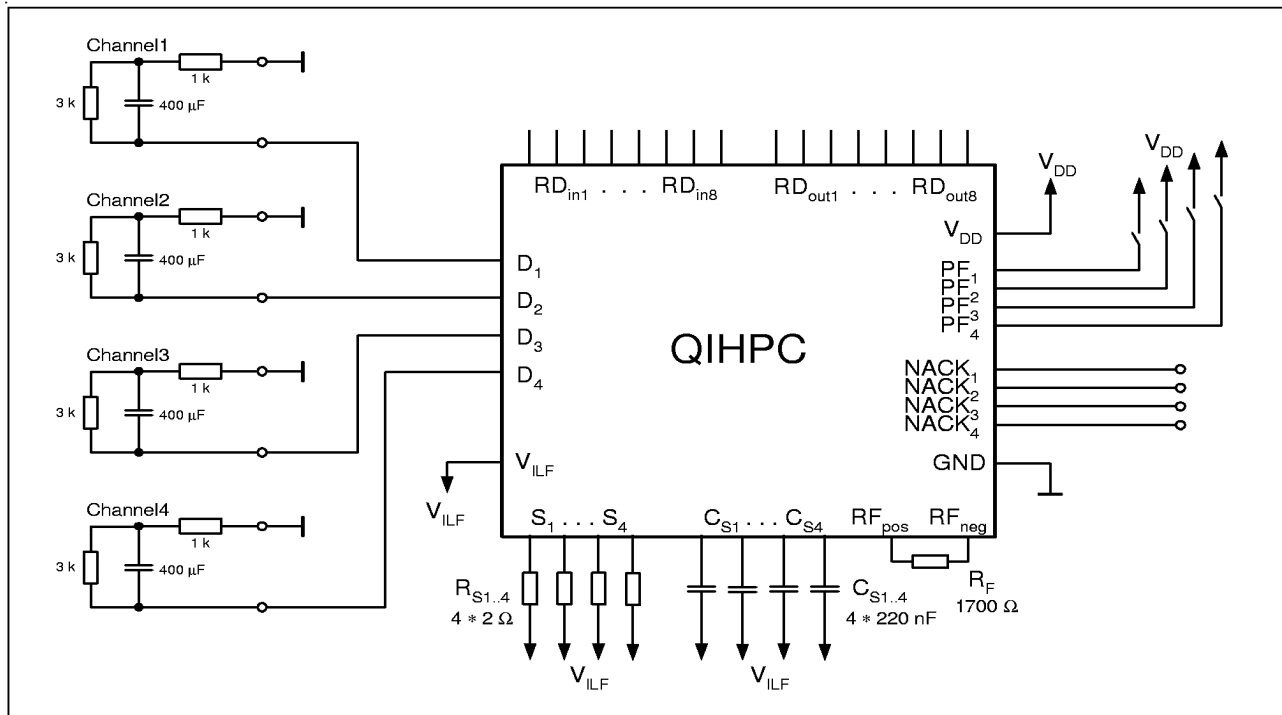
Figure 8 Circuit with “LT Power Source Test Loads”
