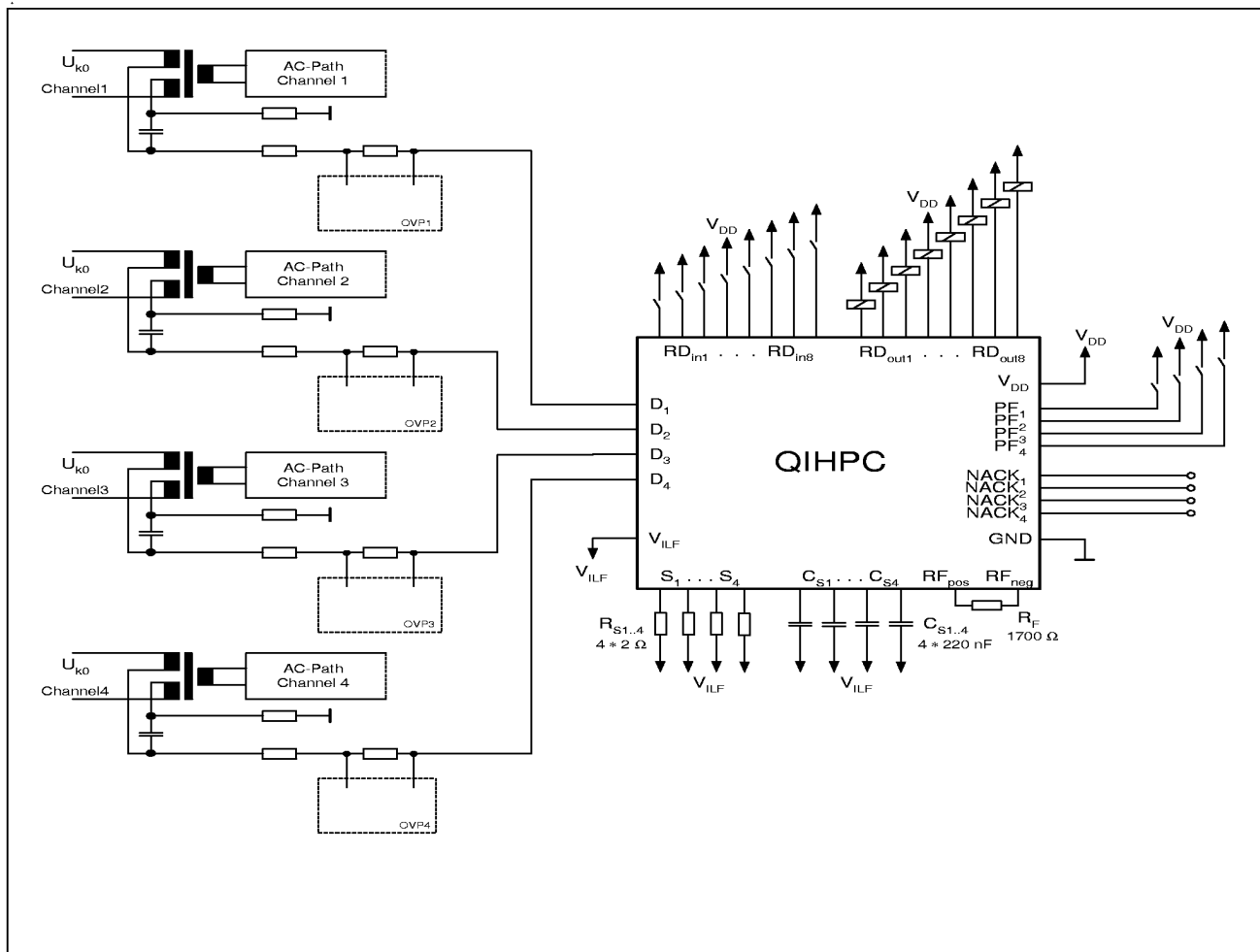
Figure 3 System integration
