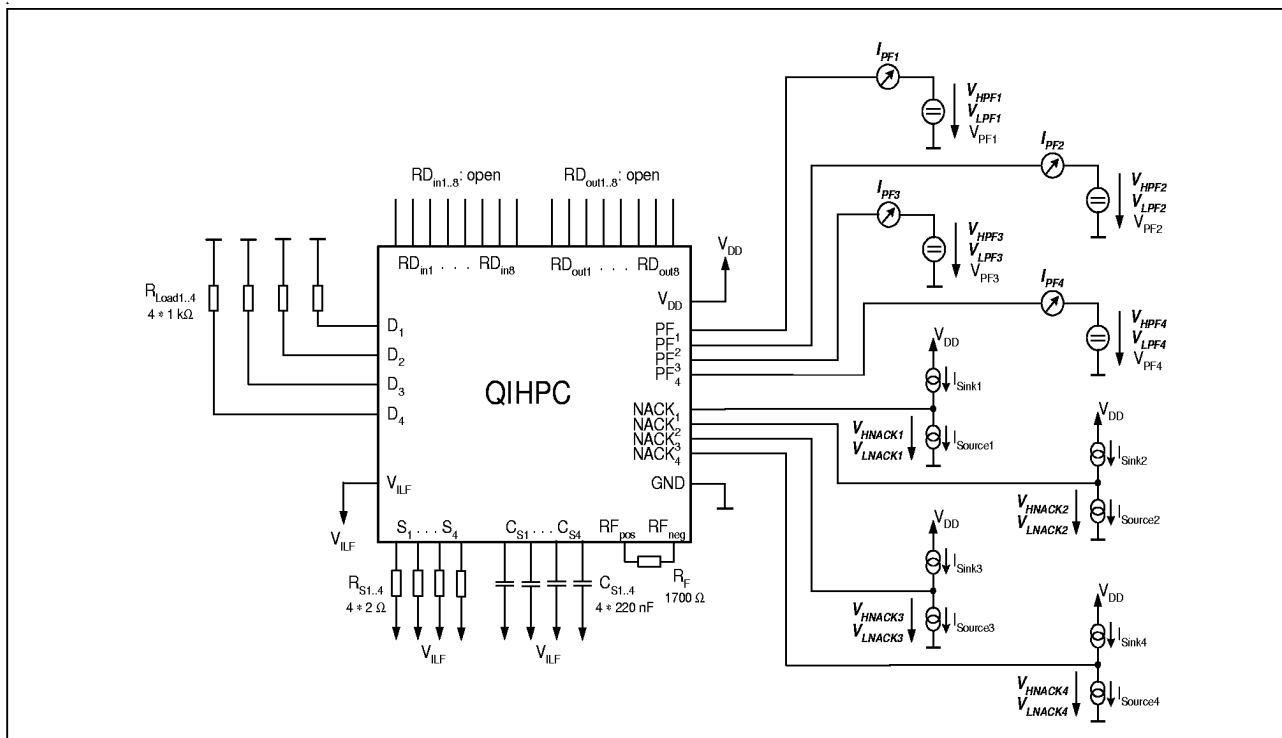
Figure 13 PF 1..4 , Logic Input Levels and NACK 1..4 , Logic Output Levels
