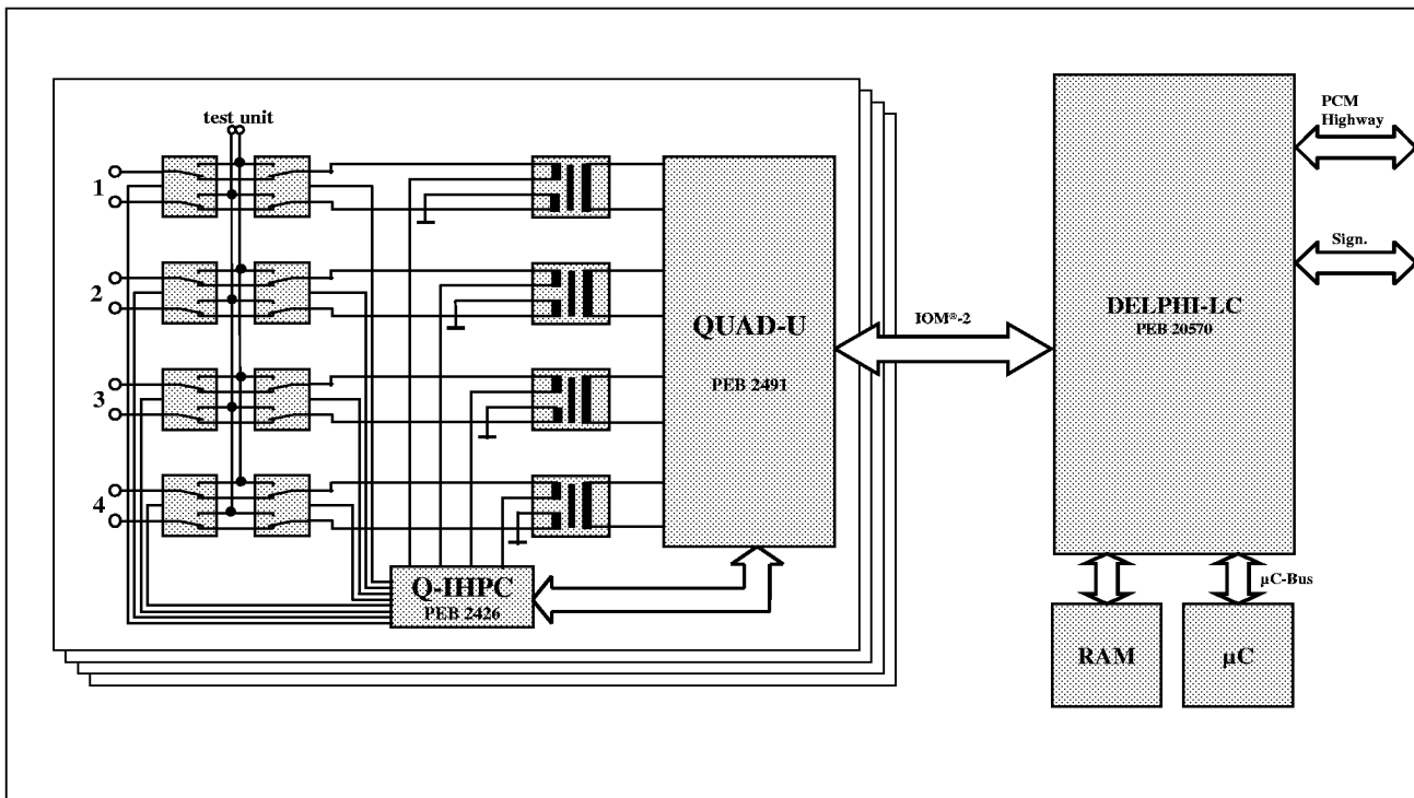
Figure 2 16-Line Card Application with DELPHI and QUAD-U
