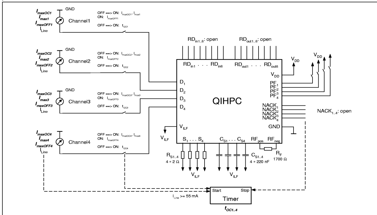
Figure 11 Line Currents and Delay Time t_{OC}
