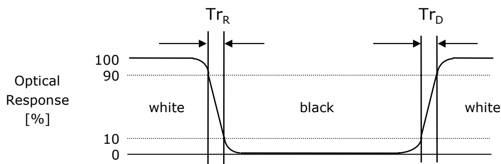
FIG. 9 Response Time
