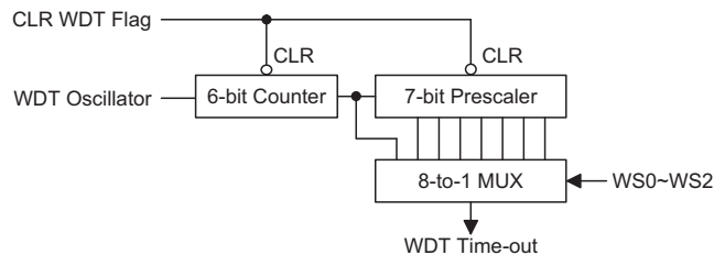
Watchdog Timer
