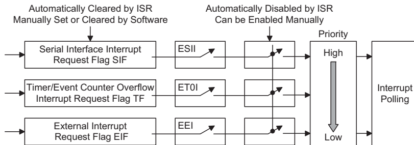
Interrupt Structure
