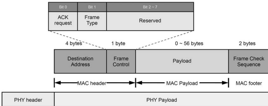
Data Frame
