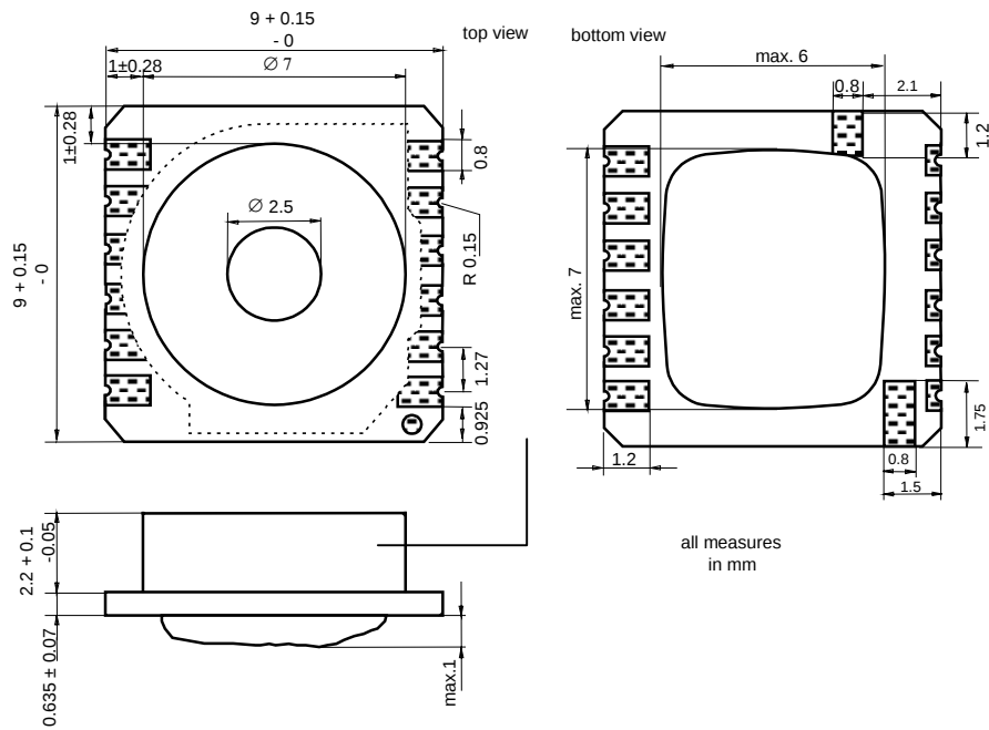
Fig. 9: Device package outlines of MS5534AP
