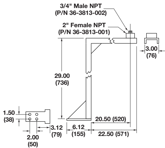
Floor Mount Bracket
