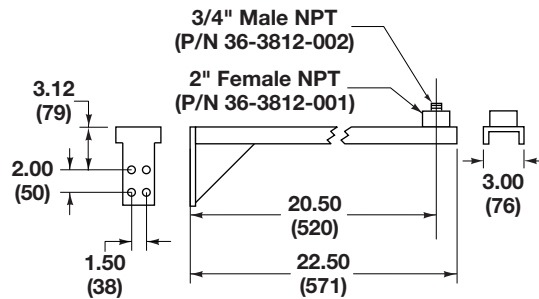
Wall Mount Bracket
