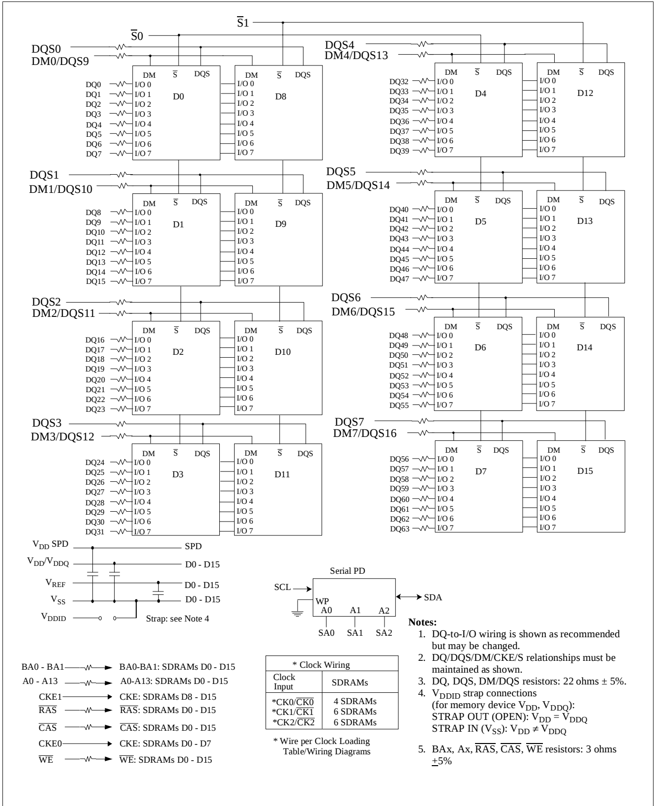
Figure 2 Block Diagram - Two Rank 64M \times 64 DDR SDRAM SO-DIMM HYS64D64020GBDL-[5/6/7/8]-B
