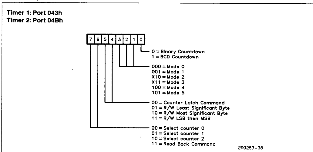
Figure 7-1. Control Word
