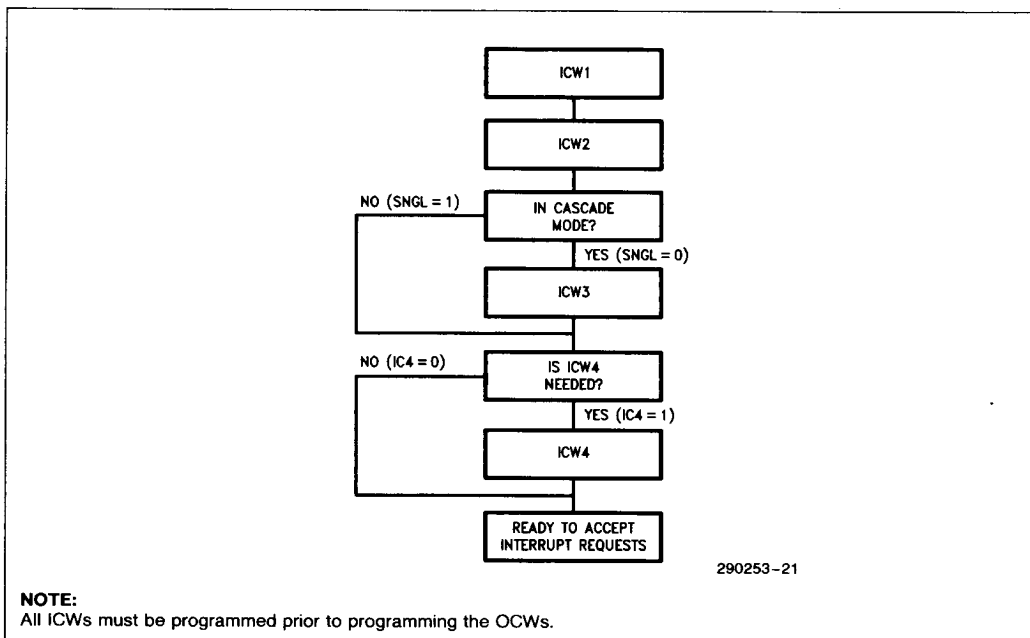
Figure 5-2. Initialization Sequence
