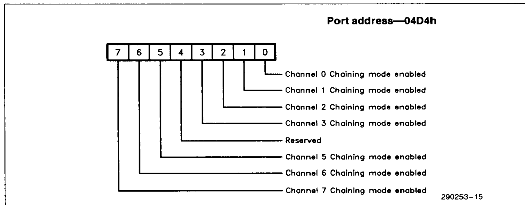
Figure 3-12. Set Chaining Mode Status Register (Read Only)
