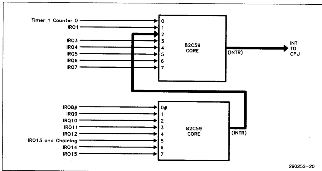
Figure 5-1. Interrupt Controller
