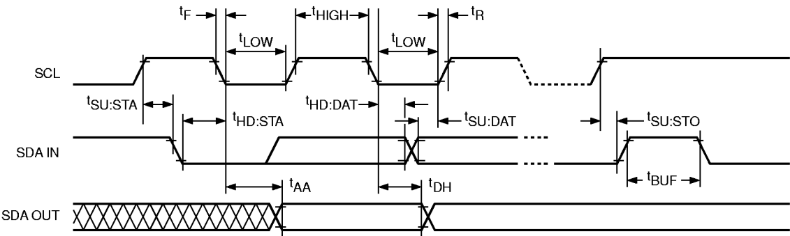
Figure 1. Bus Timing
