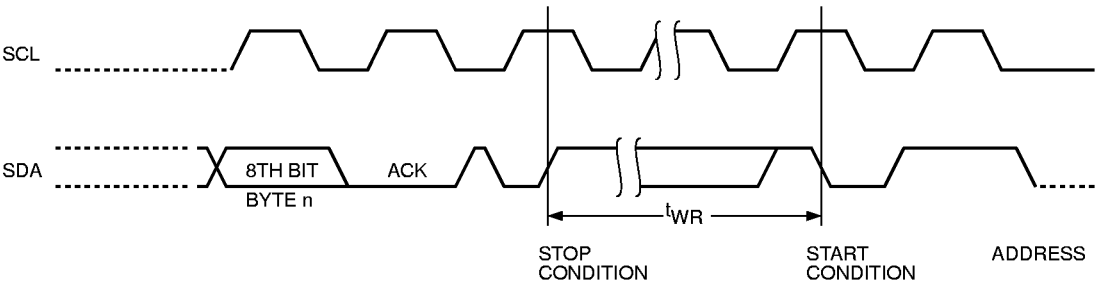
Figure 3. Start/Stop Timing
