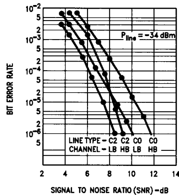
FIGURE 2. Bit Error Rate vs Signal-to-Noise Ratio
