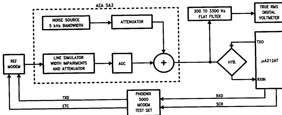
FIGURE 3. 2-Wire Bit Error Test Setup
