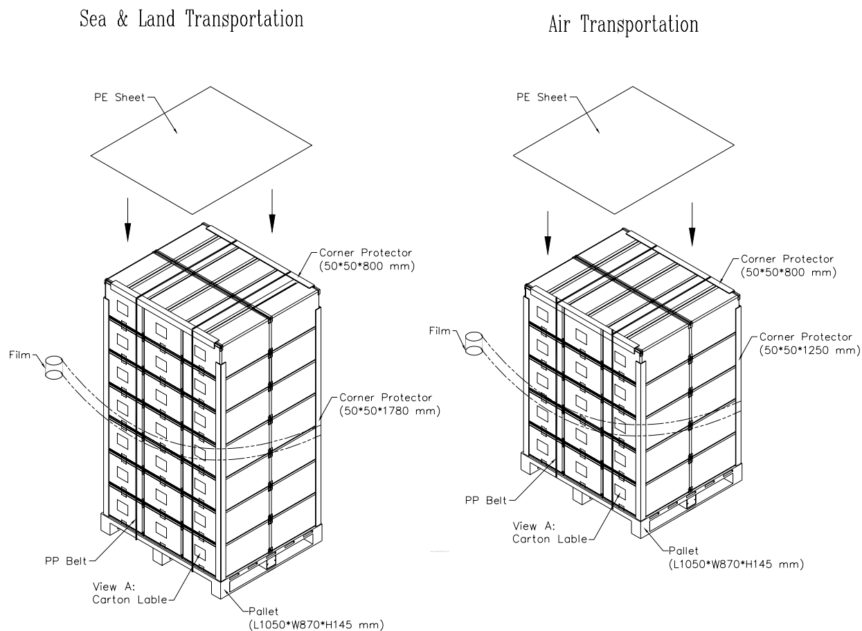
Figure. 10-2 Packing method
