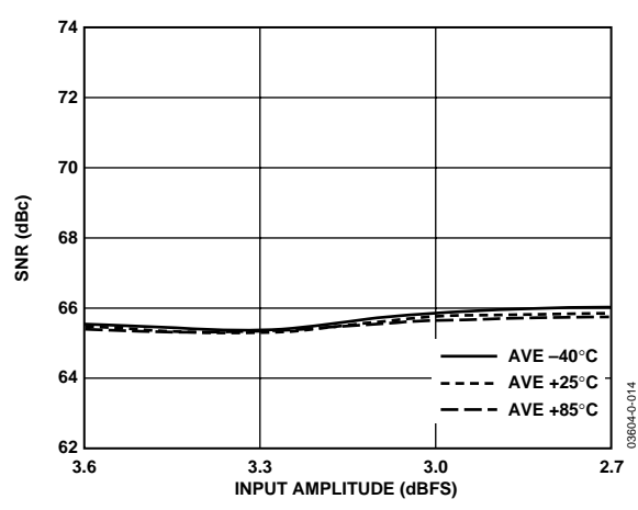
Figure 17. AD9863 Rx Path at 50 MSPS, 10 MHz Input Tone SNR Performance vs. ADC_AVDD and Temperature
