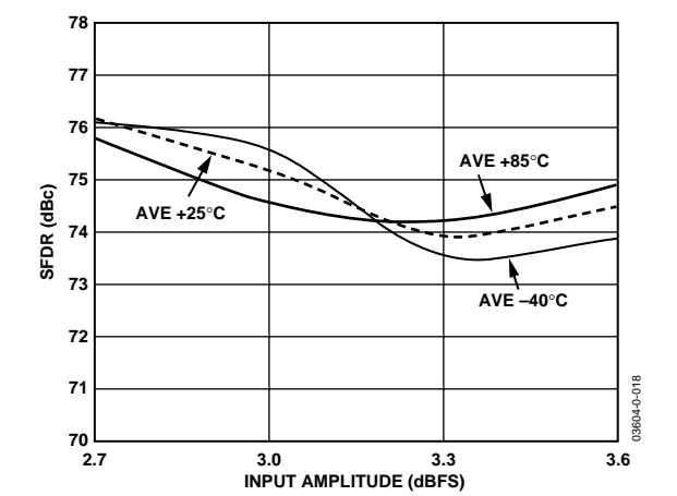
Figure 21. AD9863 Rx Path Single-Tone SFDR Performance vs. ADC_AVDD and Temperature
