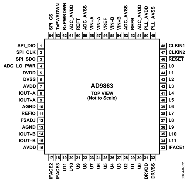
Figure 3. Pin Configuration
