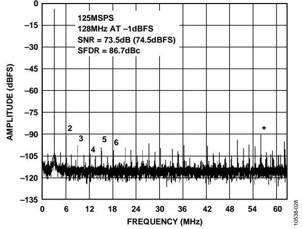
Figure 28. Single-Tone 16k FFT with f_{IN} = 128 MHz , f_{SAMPLE} = 125 MSPS , V_{REF} = 1.3 V
