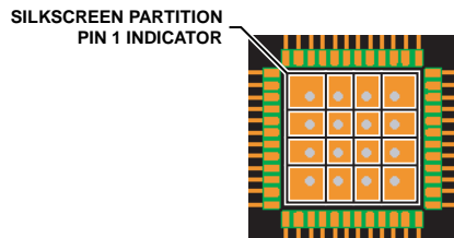
Figure 76. Typical PCB Layout
