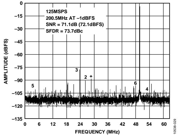
Figure 29. Single-Tone 16k FFT with f_{IN} = 200.5 MHz , f_{SAMPLE} = 125 MSPS , V_{REF} = 1.3 V
