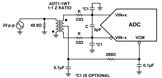
Figure 57. Differential Transformer-Coupled Configuration for Baseband Applications
