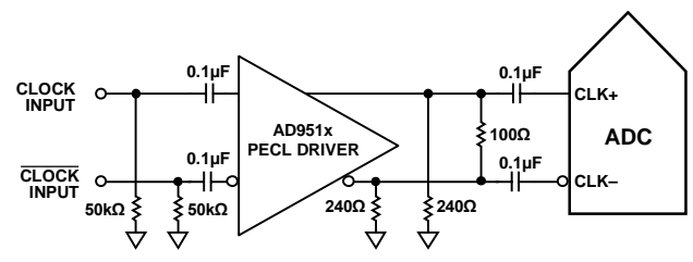
Figure 64. Differential PECL Sample Clock (Up to 1 GHz)
