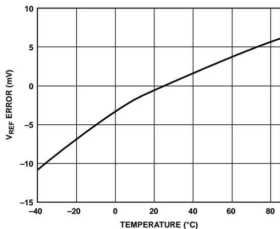
Figure 61. Typical V_{REF} = 1.3 V Drift
