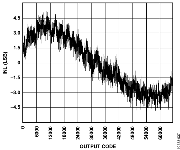
Figure 37. INL, f_{IN} = 9.7 MHz, f_{SAMPLE} = 125 MSPS, V_{REF} = 1.3 V
