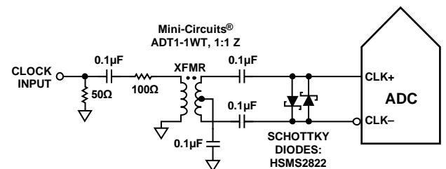
Figure 62. Transformer-Coupled Differential Clock (Up to 200 MHz)
