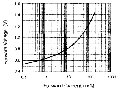
Forward Characteristics
