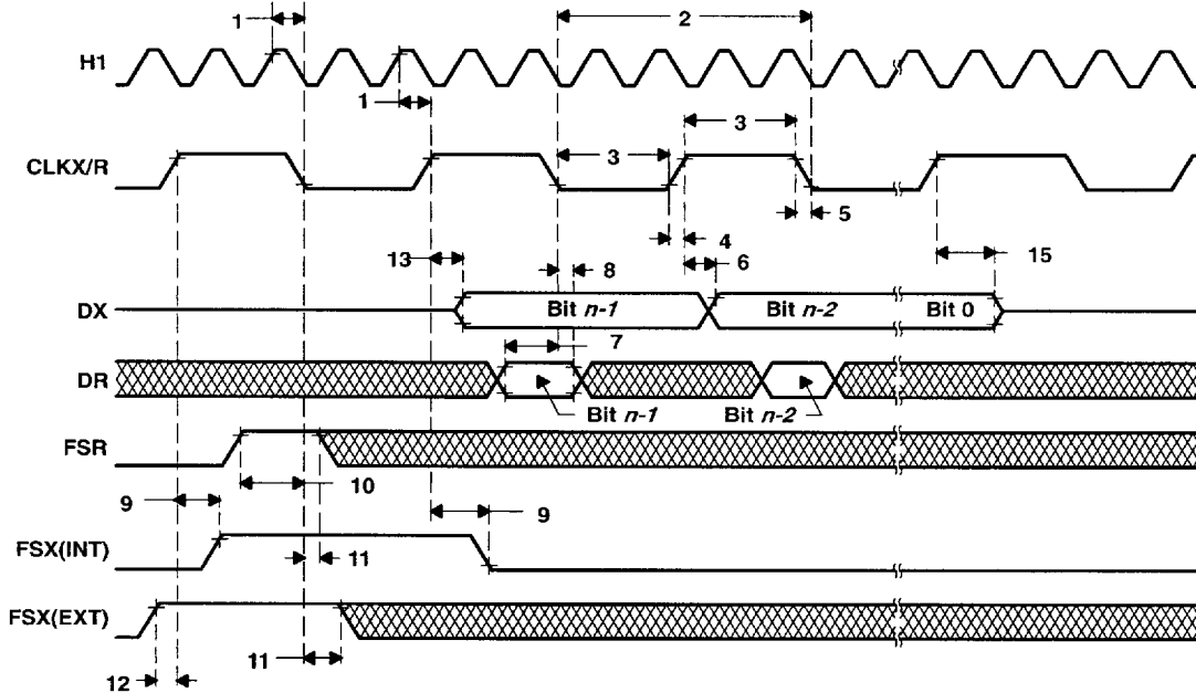
Figure 24. Timing for Fixed Data-Rate Mode
