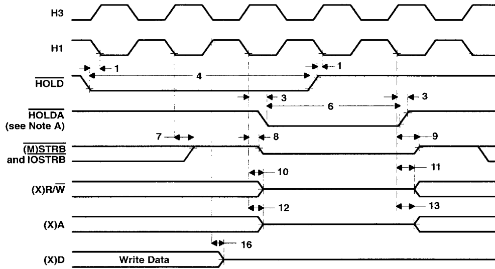
Figure 26. Timing for \overline{\text{HOLD}}/\overline{\text{HOLDA}}
