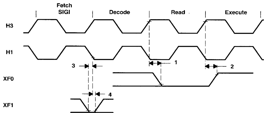
Figure 15. Timing for XF0 and XF1 When Executing SIGI
