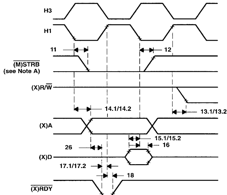
Figure 9. Timing for Memory [ (\overline{M})\text{STRB} = 0 ] Read
