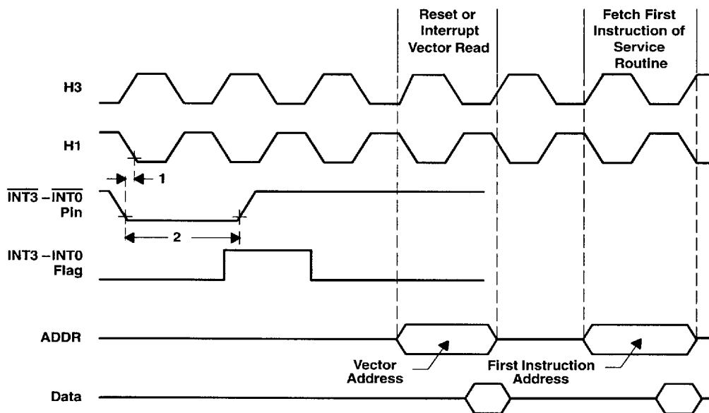
Figure 22. Timing for \overline{\text{INT3}}-\overline{\text{INT0}} Response
