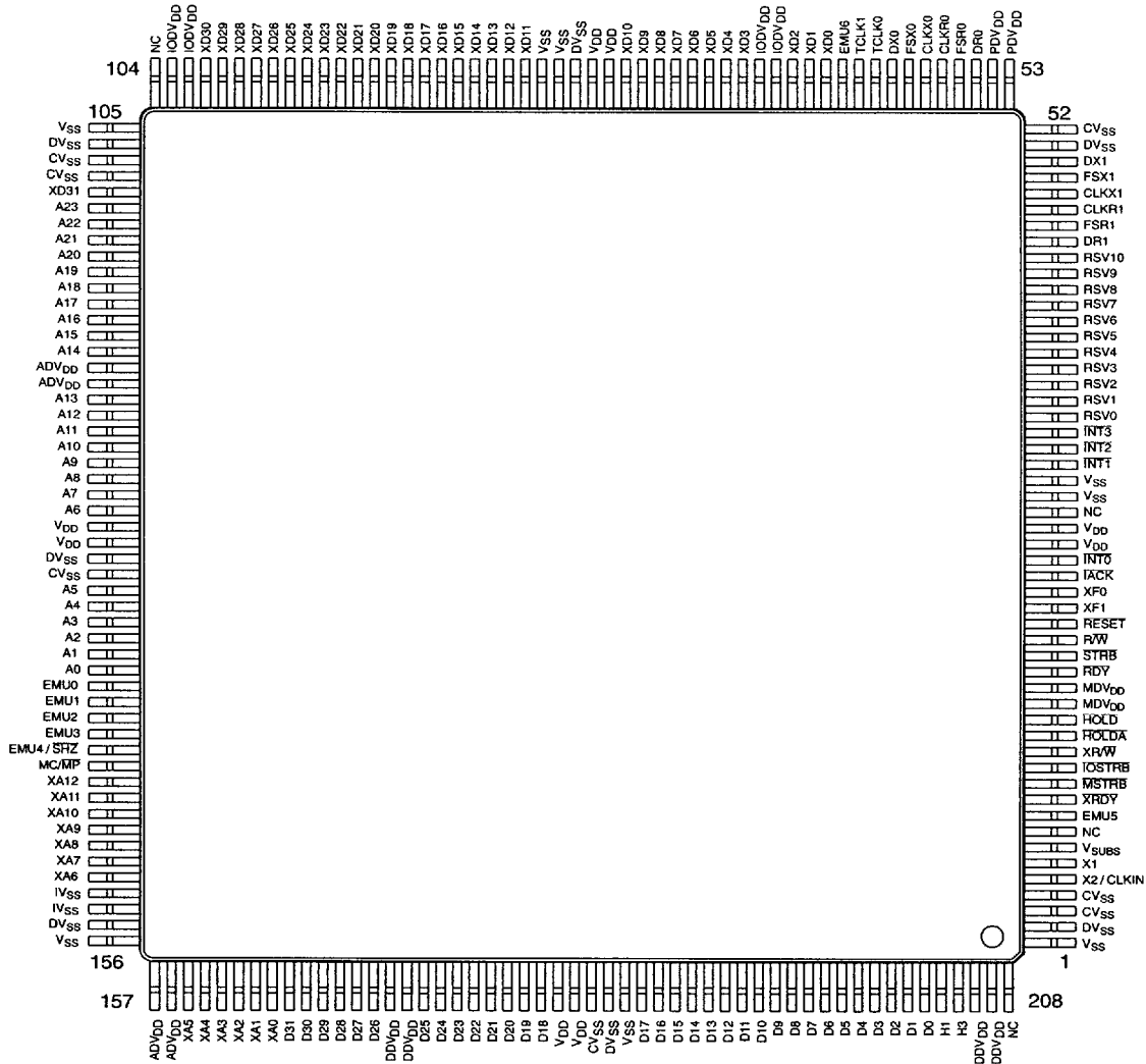
TMS320C30 PPM Pinout
