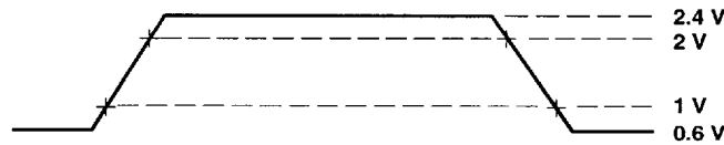
Figure 5. TTL-Level Outputs
