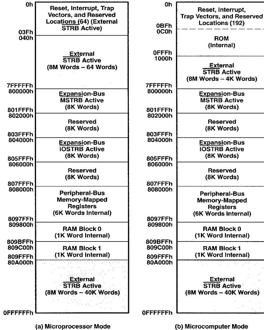
Figure 1. TMS320C30 Memory Map
