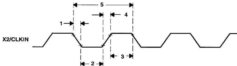
Figure 7. Timing for X2/CLKIN
