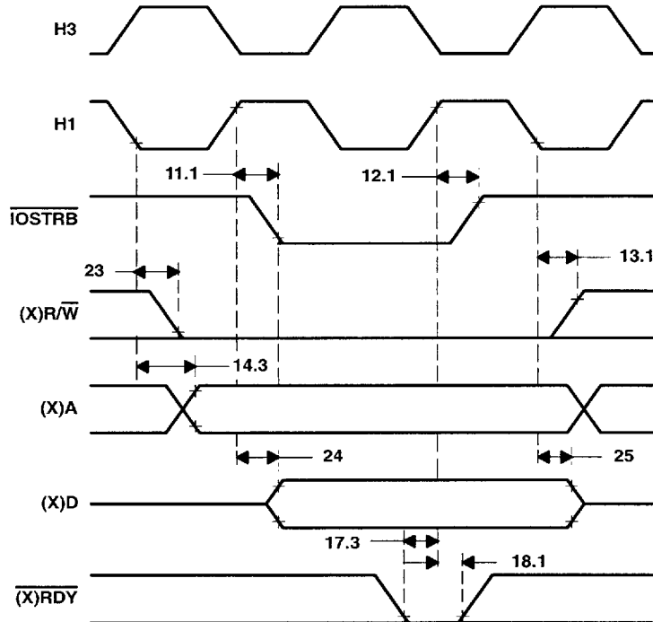
Figure 12. Timing for Memory ( \overline{\text{IOSTRB}} = 0 ) Write
