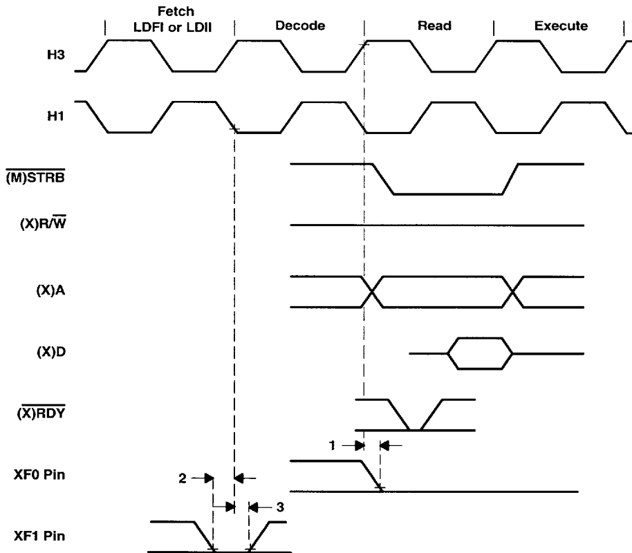
Figure 13. Timing for XF0 and XF1 When Executing LDFI or LDII
