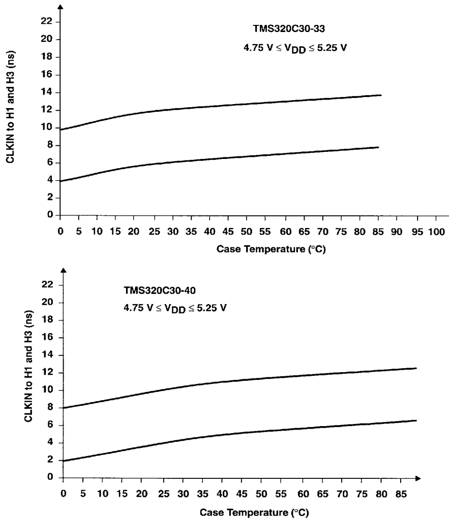
Figure 20. CLKIN to H1 and H3 as a Function of Temperature
