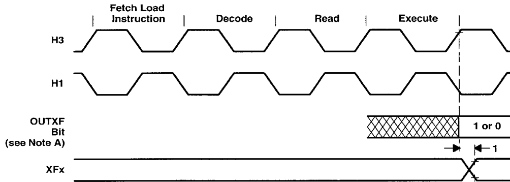
Figure 16. Timing for Loading XFx Register When Configured as an Output Pin
