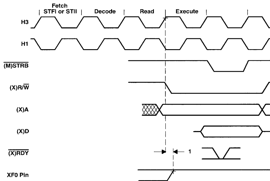
Figure 14. Timing for XF0 When Executing an STFI or STII
