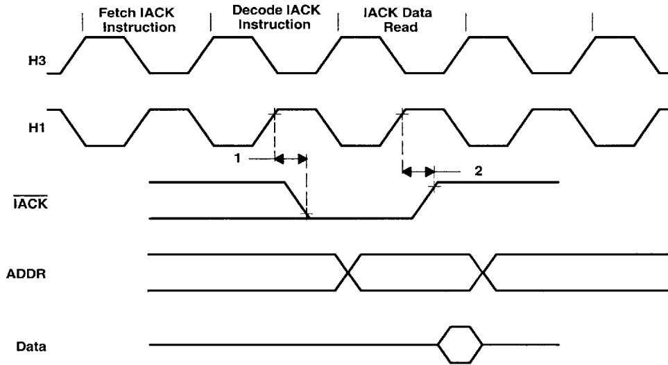
Figure 23. Timing for \overline{\text{IACK}}
