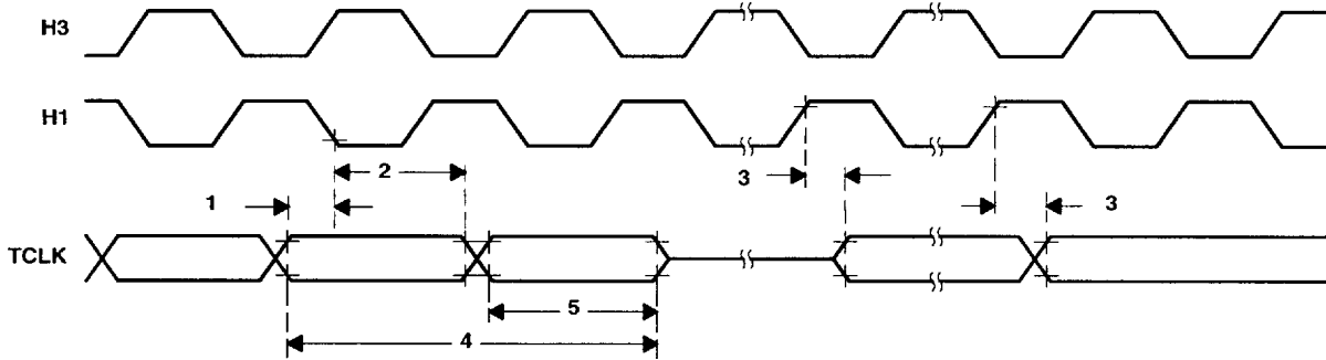
Figure 30. Timing for Timer Pin
