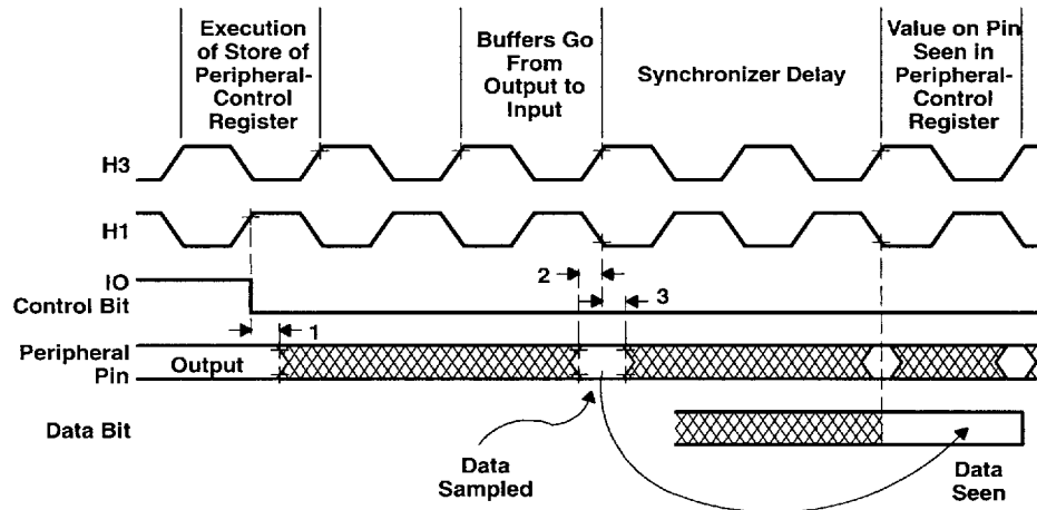
Figure 28. Timing for Change of Peripheral Pin From General-Purpose Output to Input Mode
