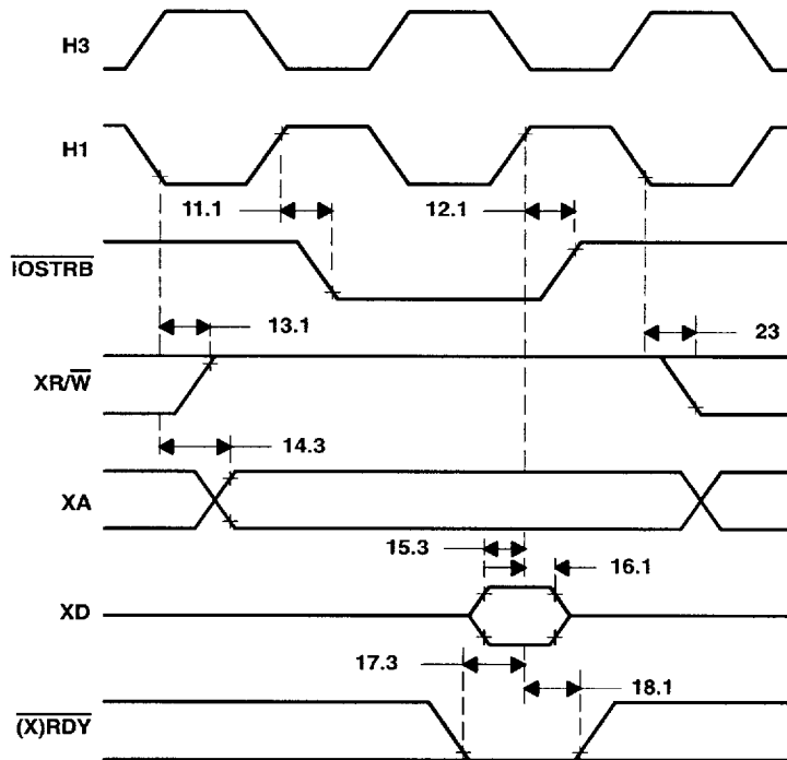
Figure 11. Timing for Memory ( \overline{\text{IOSTRB}} = 0 ) Read
