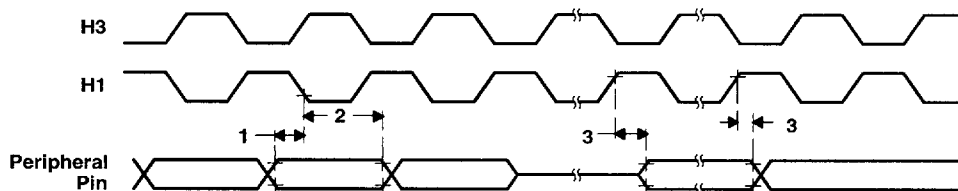
Figure 27. Timing for Peripheral Pin General-Purpose I/O
