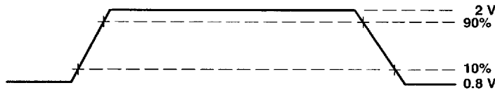
Figure 6. TTL-Level Inputs
