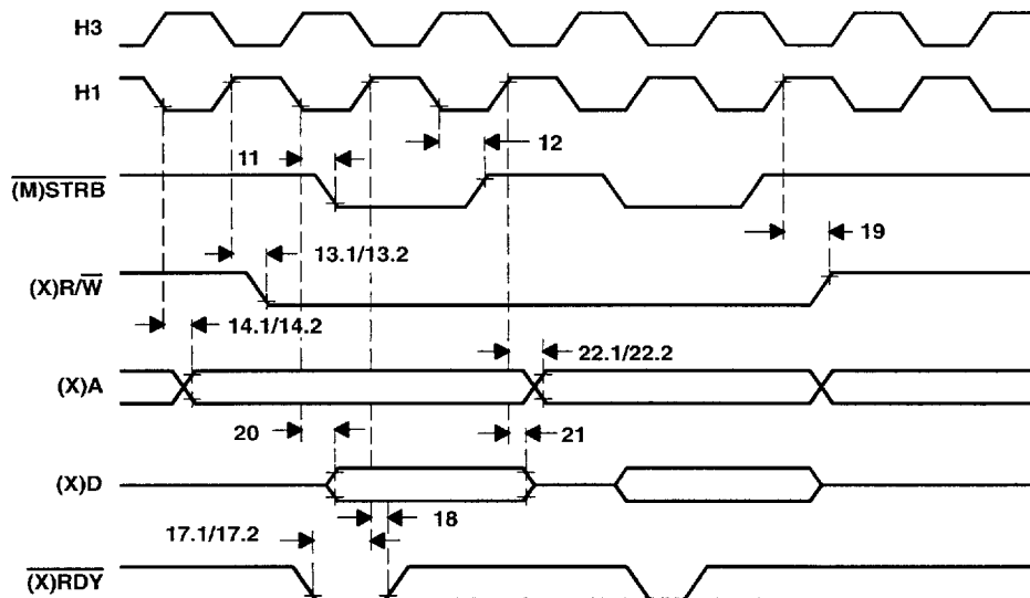
Figure 10. Timing for Memory [ (\overline{M})\text{STRB} = 0 ] Write
