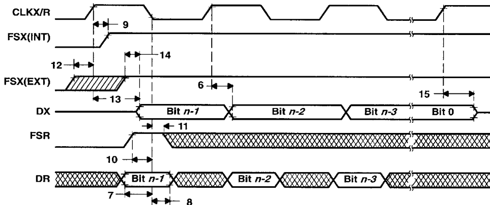
Figure 24. Timing for Fixed Data-Rate Mode
