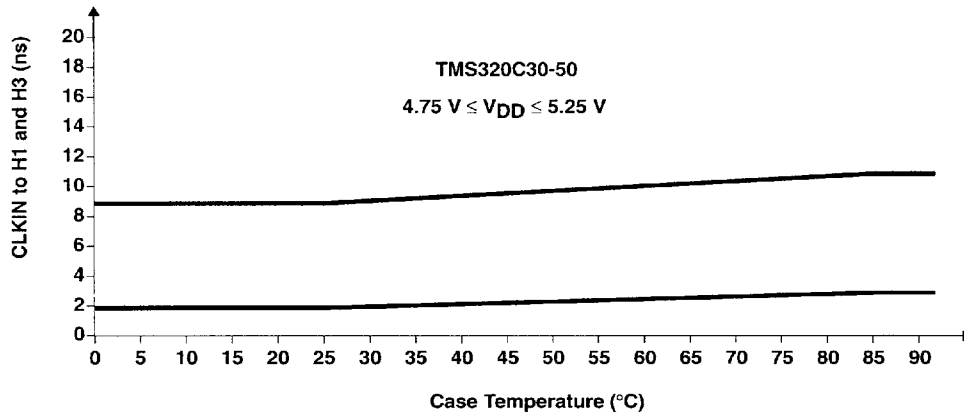
Figure 21. CLKIN to H1 and H3 as a Function of Temperature
