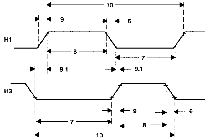
Figure 8. Timing for H1 and H3
