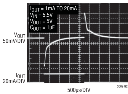
Transient Response
