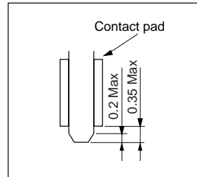
Detail D
