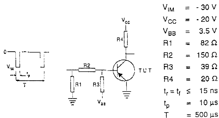
Fig. 2 Switching times test circuit.
