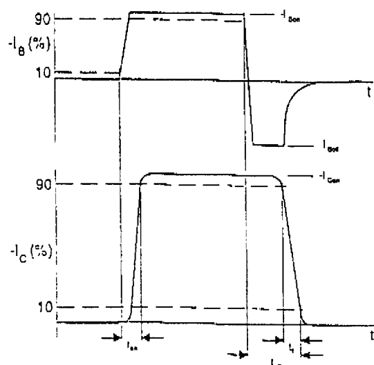
Fig. 1 Switching times waveforms.
