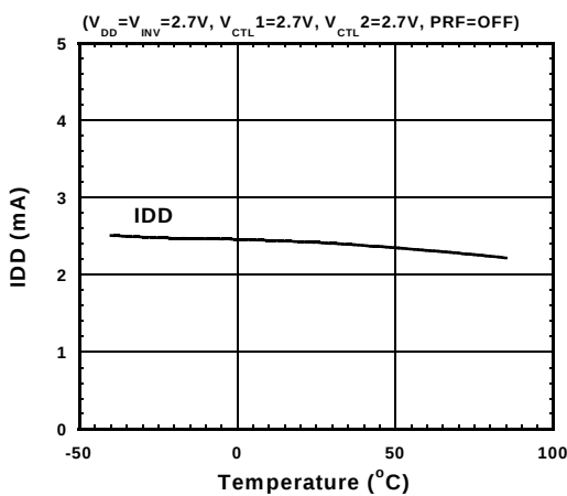
IDD vs. Temperature
