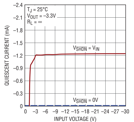
LT3015-3.3 Quiescent Current
