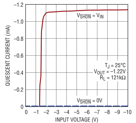
LT3015 Quiescent Current
