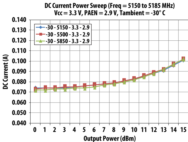
Figure 11. DC Current Power Sweep at Vcc = 3.3 V and -30° C over Frequency
