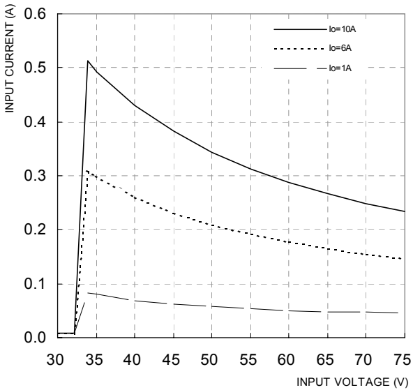
Figure 3: Typical input characteristics at room temperature.
