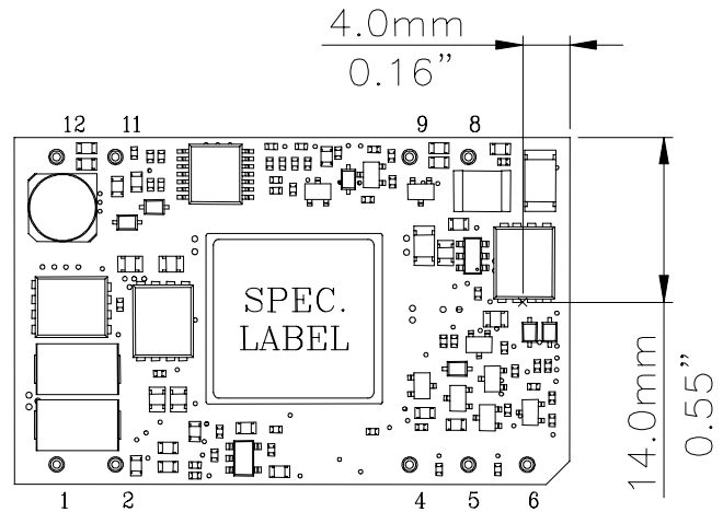
Figure 18: Hot spot temperature measured point *The allowed maximum hot spot temperature is defined at 102 °C
