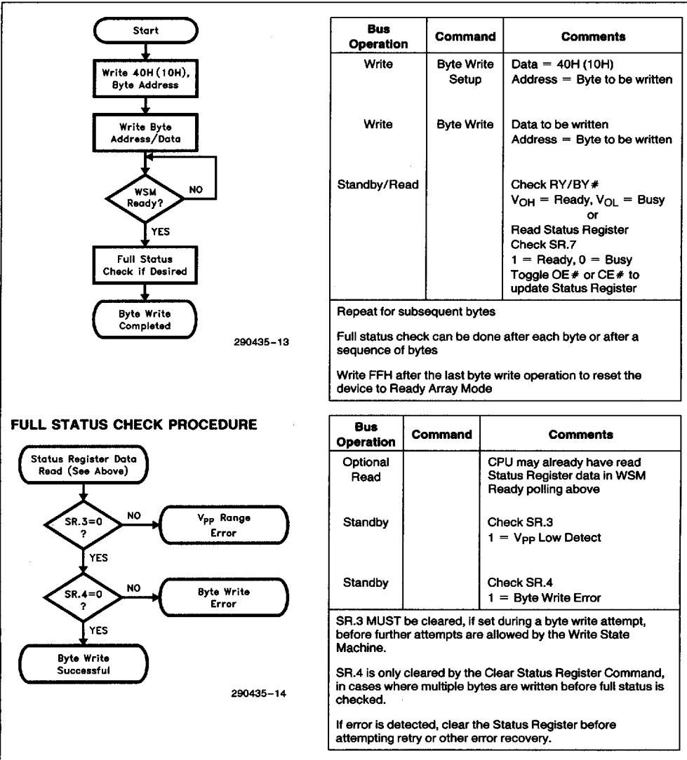
Figure 6. Automated Byte Write Flowchart
