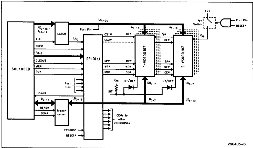
Figure 4. 28F008SA-L Array Interface to Intel3.3V 80L186EB Embedded Microprocessor
