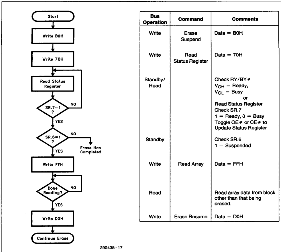
Figure 8. Erase Suspend/Resume Flowchart
