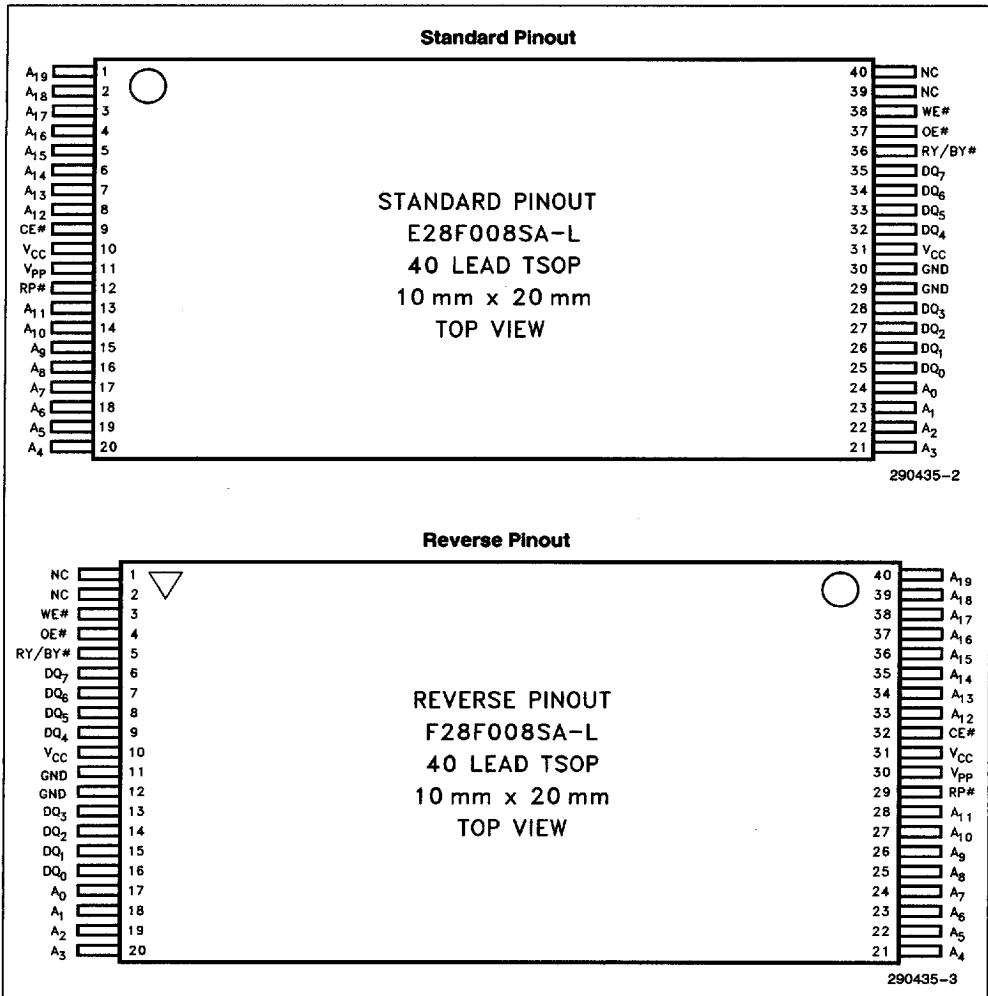
Figure 2. TSOP Lead Configurations
