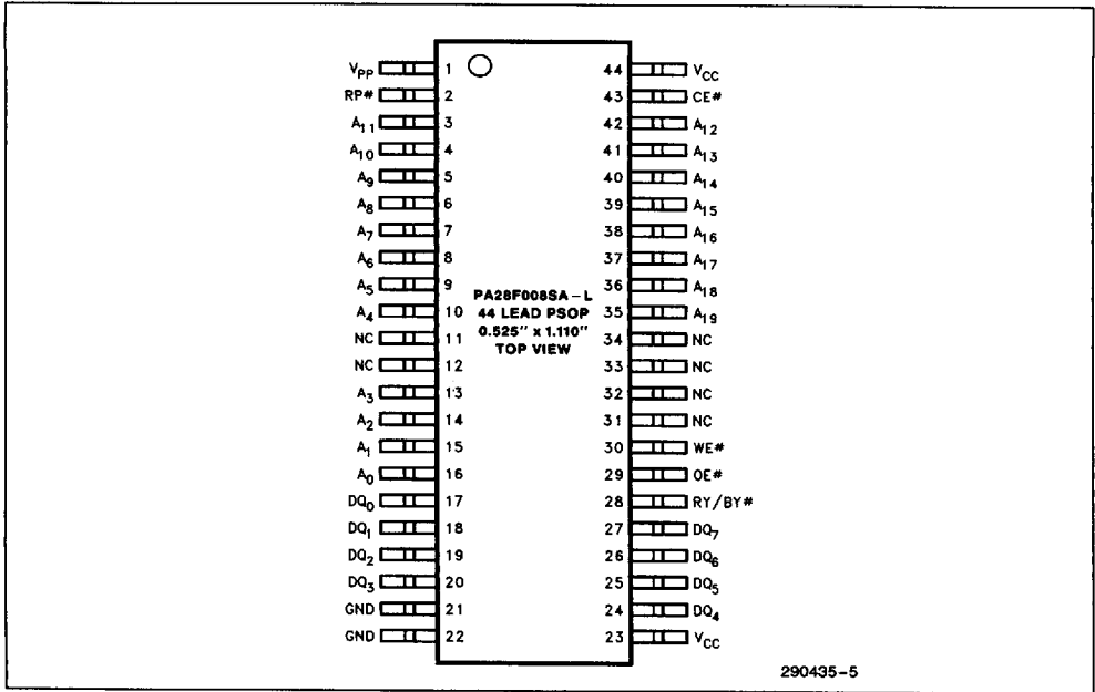
Figure 3. PSOP Lead Configuration
