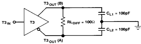
Figure 2. RS-422 Driver. Propagation Delay Test Circuit
