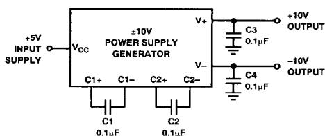
Figure 7. Charge Pump Voltage Generator
