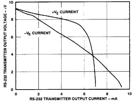
Figure 11. RS-232 Driver Output Voltage vs. Current
