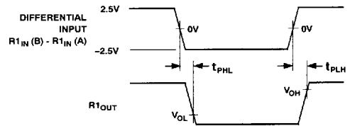
Figure 5. RS-422 Receiver Timing
