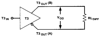
Figure 3. RS-422 Driver. Voltage Measurement Test Circuit
