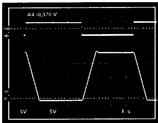
Figure 10. RS-232 Driver; R_L = 5\text{ k}\Omega , C_L = 50\text{ pF}
