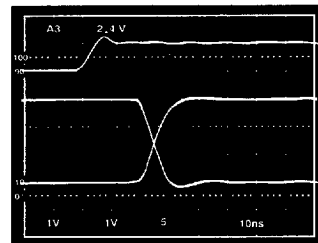
Figure 13. RS-422 Driver; R_{L,DIFF} = 100\ \Omega , C_{L1} = C_{L2} = 100\text{ pF}
