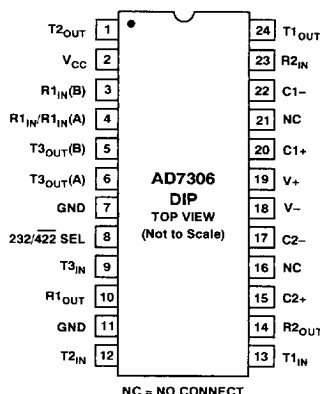
DIP Pin Configuration
