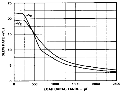
Figure 9. RS-232 Driver Slew Rate vs. Load Capacitance
