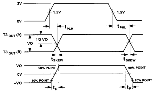
Figure 4. RS-422 Driver. Propagation Delay, Rise/Fall Timing
