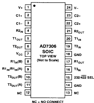
SOIC Pin Configuration
