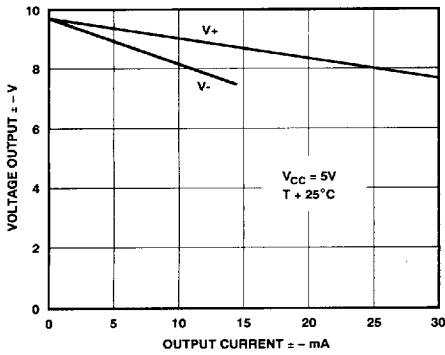
Figure 8. V_+ and V_- Voltage vs. Current
