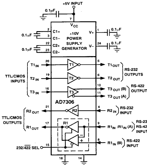
Figure 1. AD7306 Application Circuit (SOIC Package)
