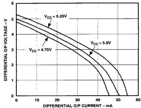
Figure 12. RS-422 Driver Output Current vs. Output Voltage
