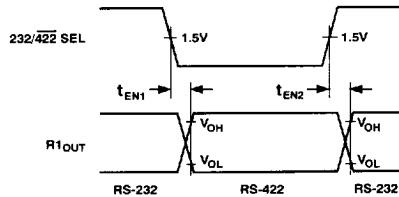
Figure 6. RS-232/RS-422 Receiver Enable Timing
