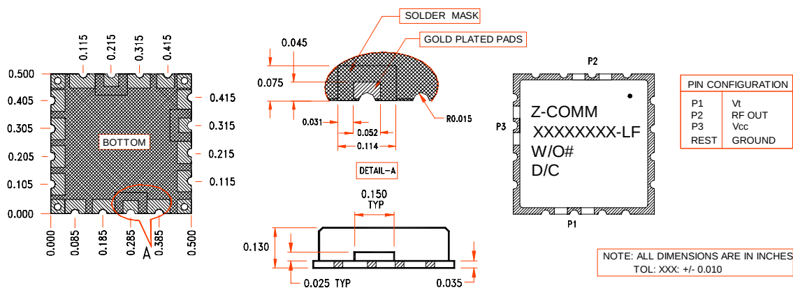
Physical Dimensions
