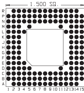
149 Pins Footprint 15018
