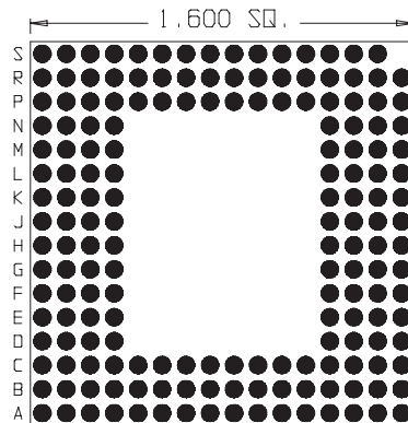
175 Pins Footprint 16008
