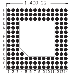
133 Pins Footprint 14013
