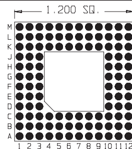
108 Pins Footprint 12004
