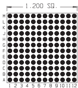
144 Pins Footprint 12001
