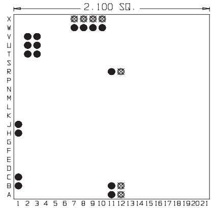
17 Pins Footprint 21009
