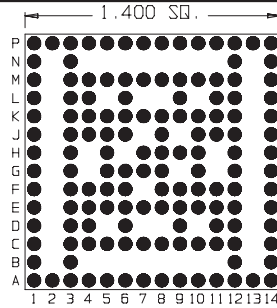
139 Pins Footprint 14010
