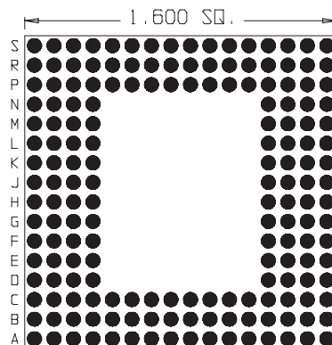
176 Pins Footprint 16007
