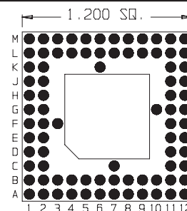
84 Pins Footprint 12010
