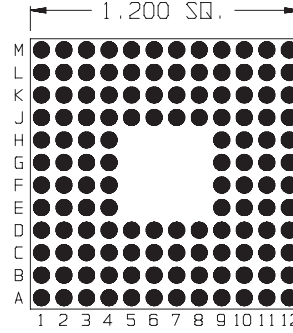
128 Pins Footprint 12025
