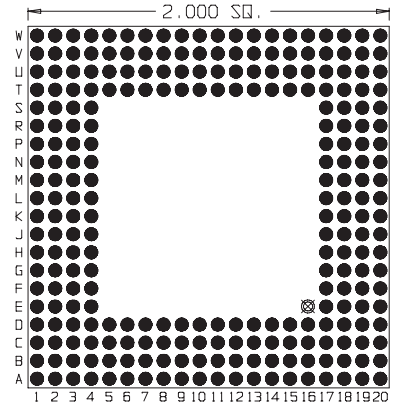
256 Pins Footprint 20017
