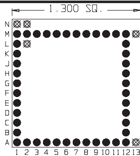
44 Pins Footprint 13090
