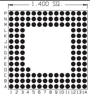
133 Pins Footprint 14014
