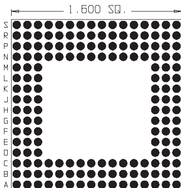
166 Pins Footprint 16004
