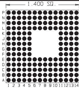
171 Pins Footprint 14008
