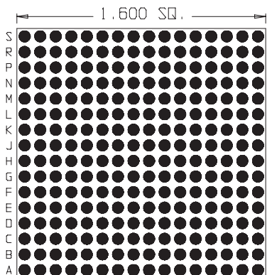
256 Pins Footprint 16001
