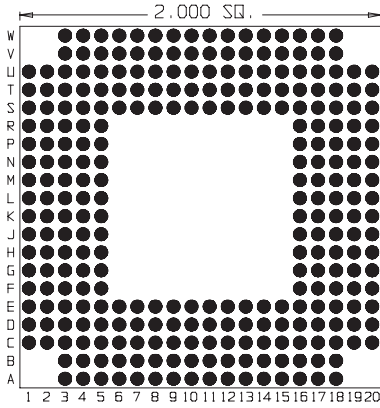
240 Pins Footprint 20010
