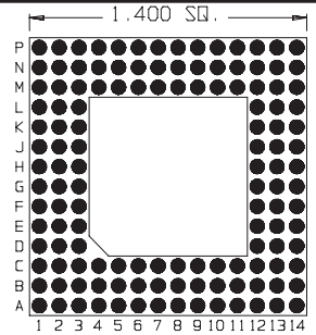
132 Pins Footprint 14015
