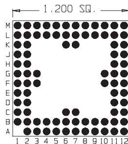
88 Pins Footprint 12009
