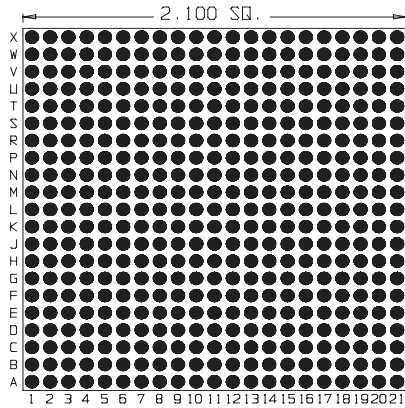
441 Pins Footprint 21001
