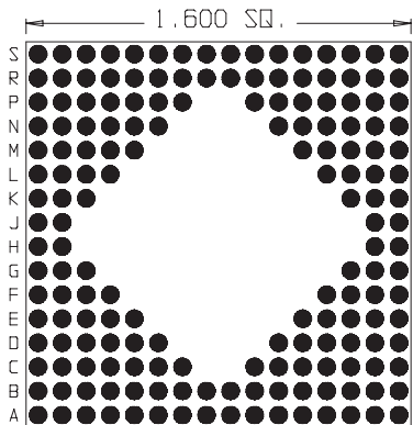
172 Pins Footprint 16002
