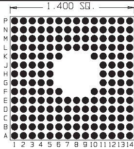
175 Pins Footprint 14006
