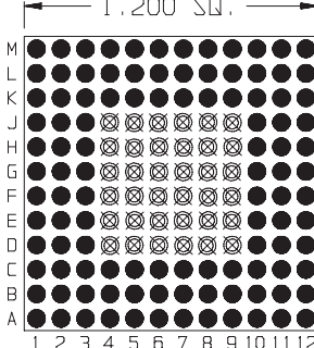
108 Pins Footprint 12024
