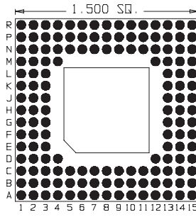
148 Pins Footprint 15021
