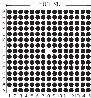
223 Pins Footprint 15003
