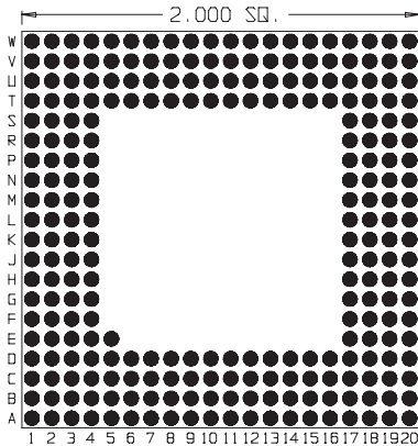
257 Pins Footprint 20012
