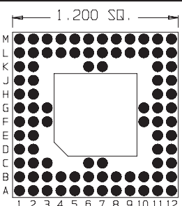
89 Pins Footprint 12006
