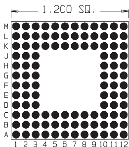
108 Pins Footprint 12005
