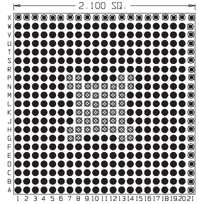
352 Pins (393) Footprint 20016
