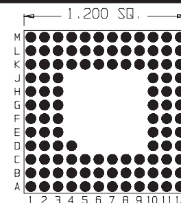
109 Pins Footprint 12003
