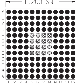
128 Pins Footprint 12023
