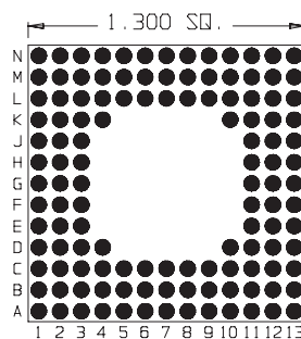
124 Pins Footprint 13009
