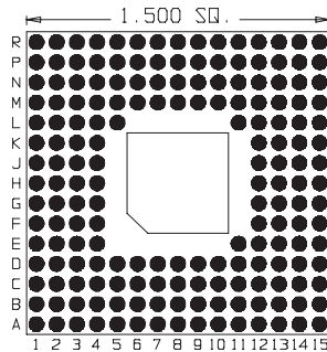
179 Pins Footprint 15011
