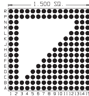
160 Pins Footprint 15015
