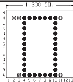
34 Pins Footprint 13091
