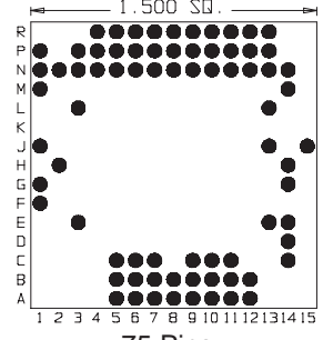
75 Pins Footprint 15032
