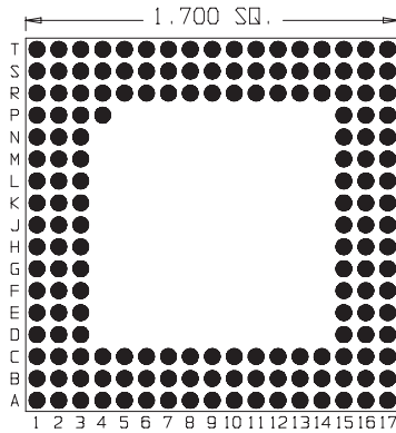
169 Pins Footprint 17002
