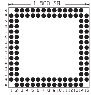
100 Pins Footprint 15031
