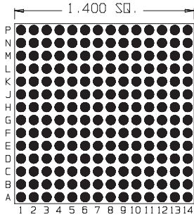
196 Pins Footprint 14001
