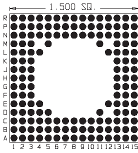
153 Pins Footprint 15017
