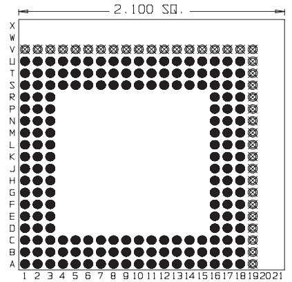
180 Pins Footprint 21007
