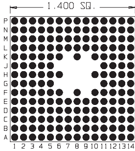
179 Pins Footprint 14005
