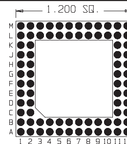
80 Pins Footprint 12014
