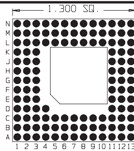
121 Pins Footprint 13012
