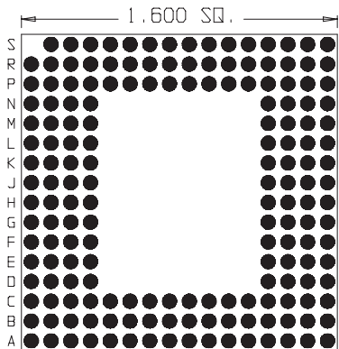
175 Pins Footprint 16003
