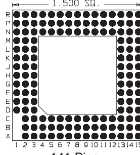
141 Pins Footprint 15028
