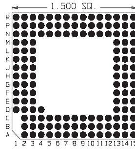
142 Pins Footprint 15027
