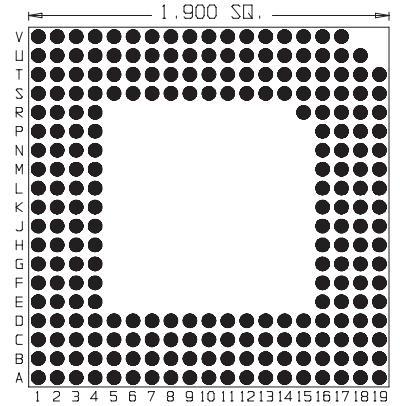
238 Pins Footprint 19007
