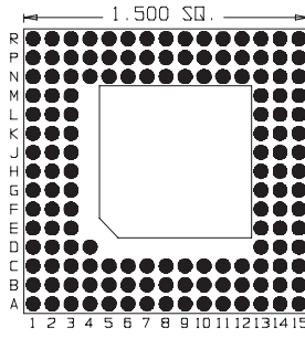
145 Pins Footprint 15023
