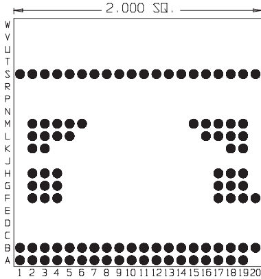
100 Pins Footprint 20011
