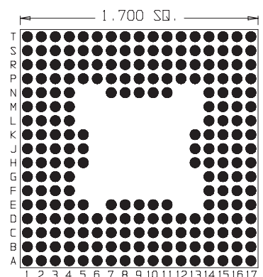
225 Pins Footprint 17007
