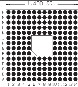
180 Pins Footprint 14002
