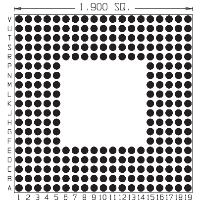
280 Pins Footprint 19006
