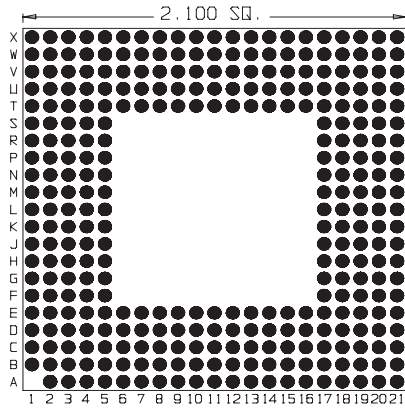
319 Pins Footprint 21002
