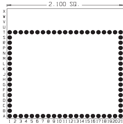
72 Pins Footprint 21003
