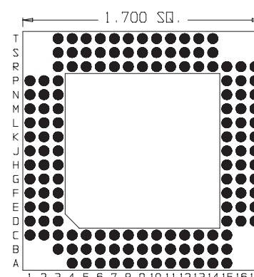
145 Pins Footprint 17003
