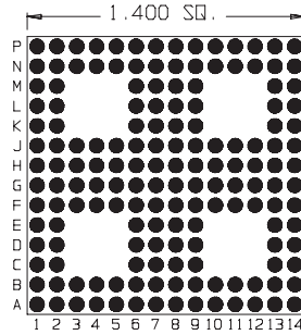
160 Pins Footprint 14009
