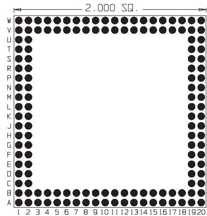
144 Pins Footprint 20007
