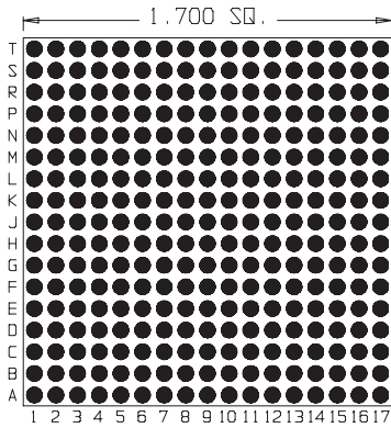
289 Pins Footprint 17001
