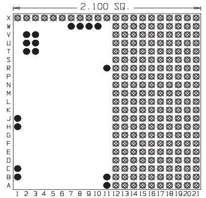
17 Pins Footprint 21008
