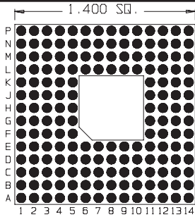
171 Pins Footprint 14007
