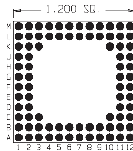
84 Pins Footprint 12013
