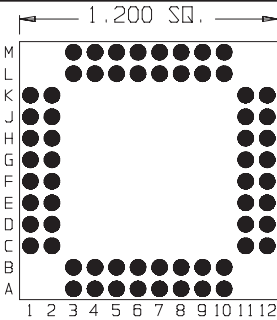
64 Pins Footprint 12018
