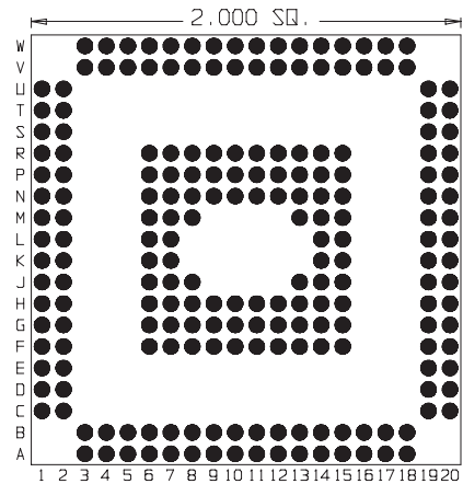
208 Pins Footprint 20008
