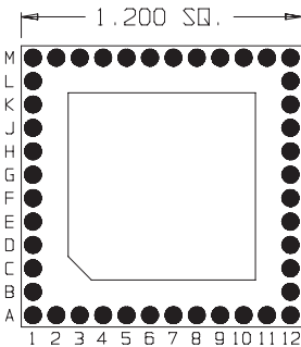
44 Pins Footprint 12019
