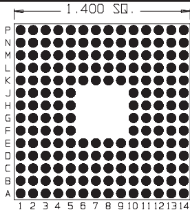
180 Pins Footprint 14003
