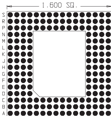
176 Pins Footprint 16006
