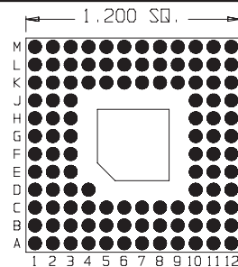
109 Pins Footprint 12002
