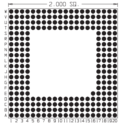
257 Pins Footprint 20018
