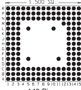
149 Pins Footprint 15020
