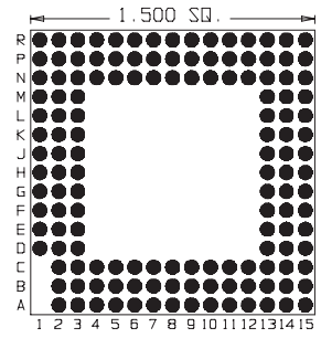
141 Pins Footprint 15029
