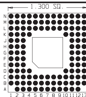
122 Pins Footprint 13010
