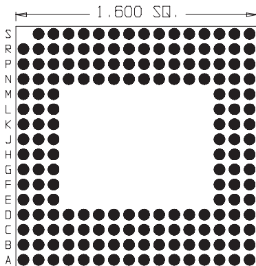
175 Pins Footprint 16005
