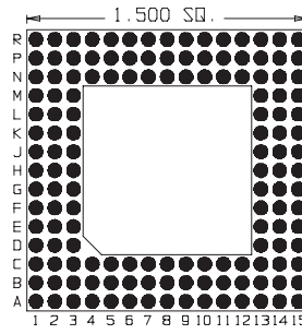
144 Pins Footprint 15025
