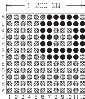
36 Pins Footprint 12020
