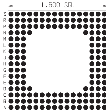
159 Pins Footprint 16009
