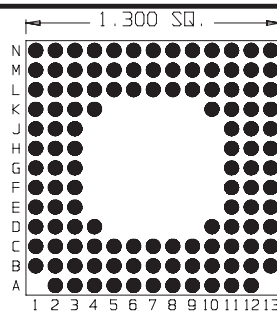
122 Pins Footprint 13011
