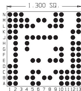
90 Pins Footprint 13089
