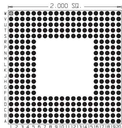
299 Pins Footprint 20009
