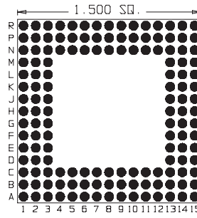
144 Pins Footprint 15026
