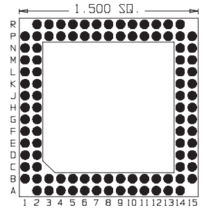
100 Pins Footprint 15030
