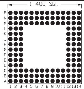
132 Pins Footprint 14016
