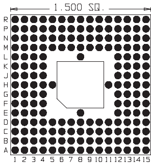
180 Pins Footprint 15007
