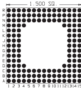
148 Pins Footprint 15022
