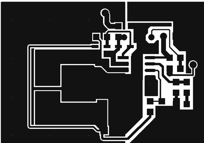
(PCB - TOP)
