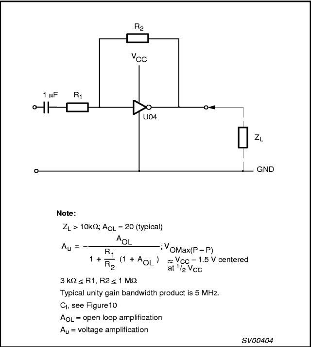
Figure 7. LVU04 used as a linear amplifier.
