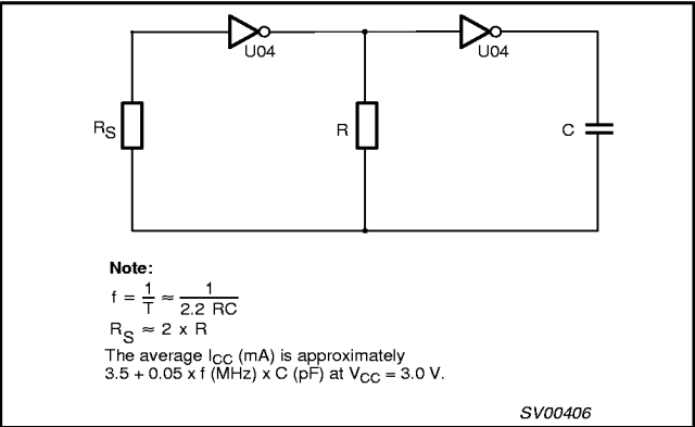
Figure 9. LVU04 used as an astable multivibrator.
