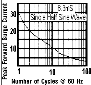
Non-Repetitive Peak Forward Surge Current
