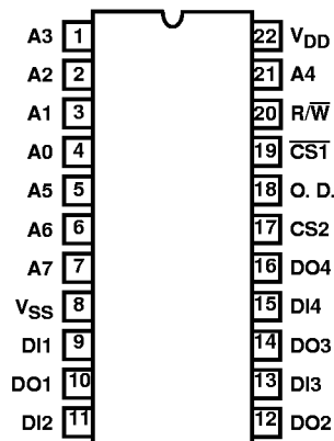
CDP1822C/3 (SBDIP) TOP VIEW
