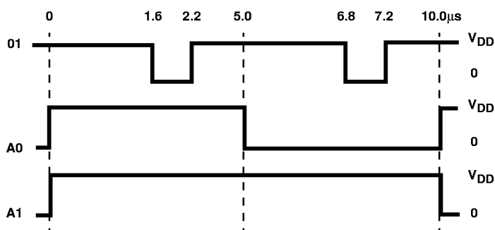
FIGURE 5. DYNAMIC/OPERATING BURN-IN CIRCUIT AND TIMING DIAGRAM
