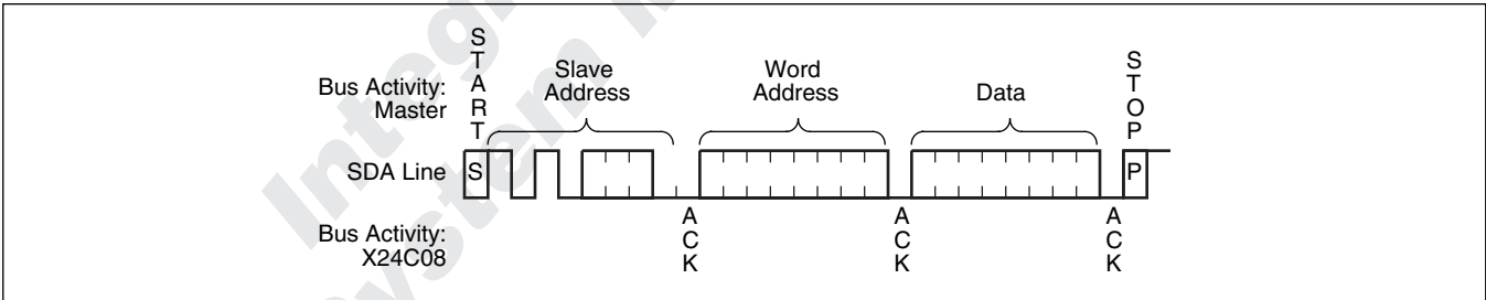
Figure 5. Byte Write
