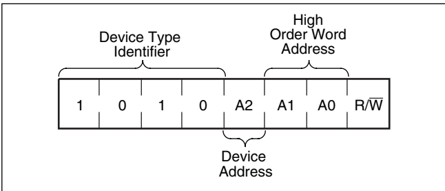
Figure 4. Slave Address
