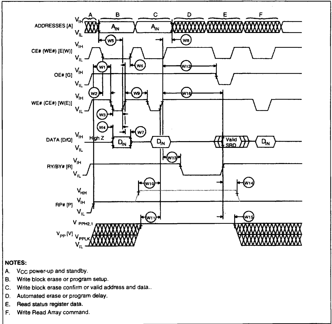
Figure 19. AC Waveform for Write Operations
