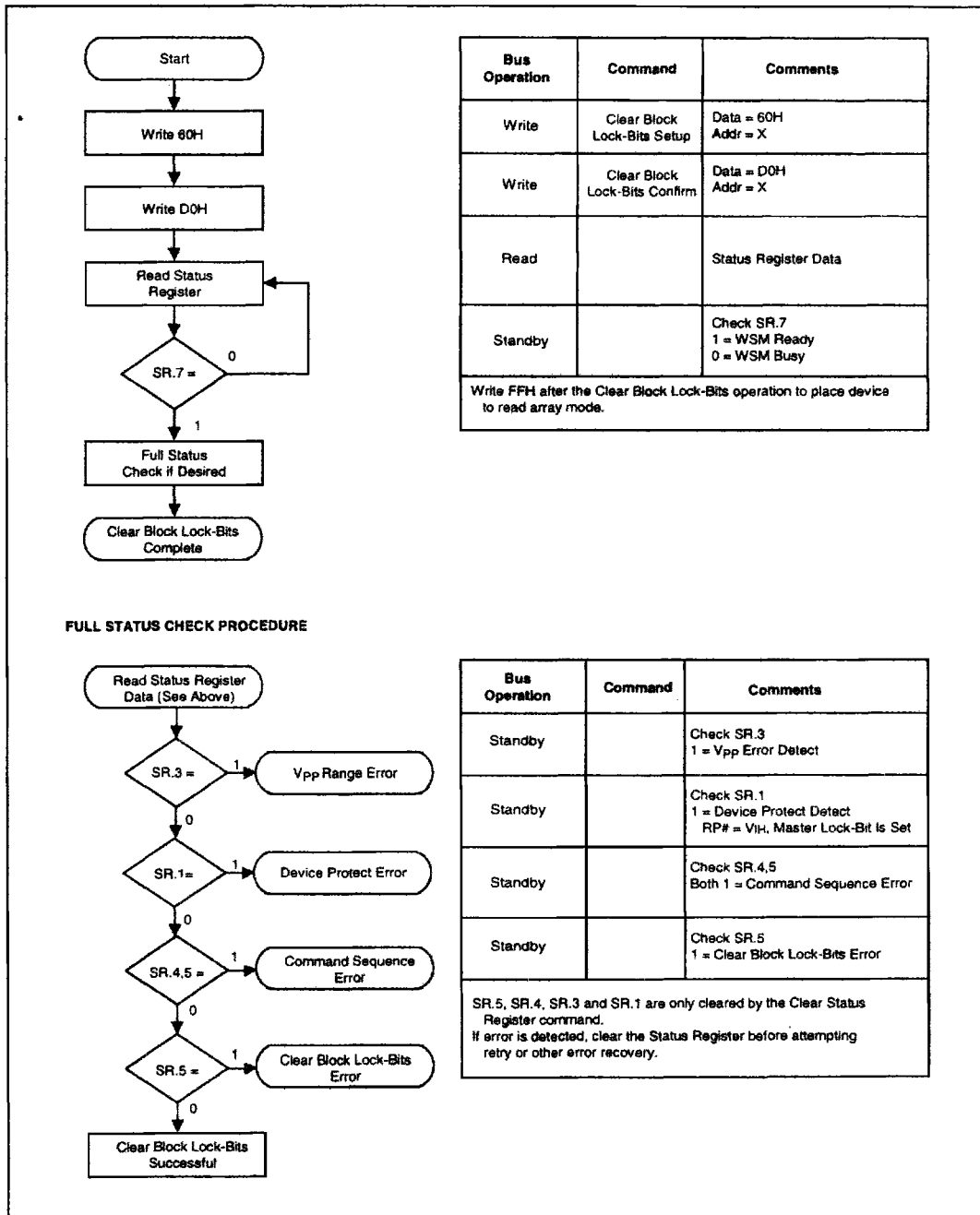
Figure 12. Clear Block Lock-Bits Flowchart
