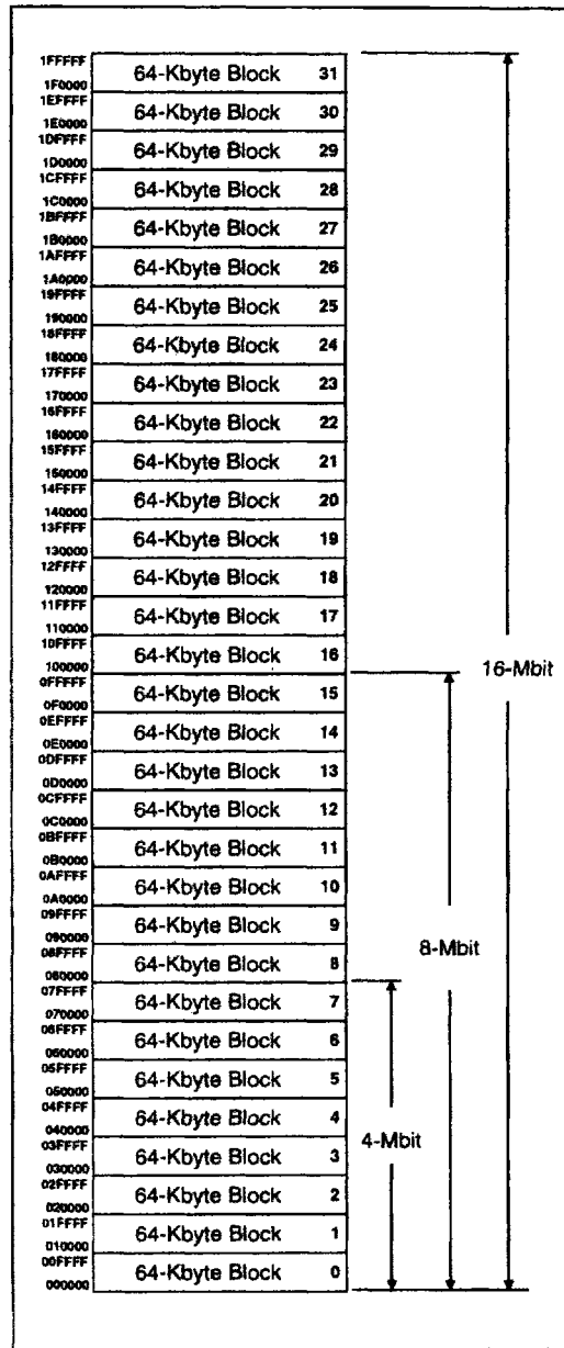
Figure 5. Memory Map
