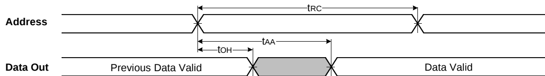
TIMING WAVEFORM OF READ CYCLE(1) (Address Controlled, \overline{\text{CS}}1=\overline{\text{OE}}=V_{\text{IL}} , \overline{\text{WE}}=V_{\text{IH}} )
