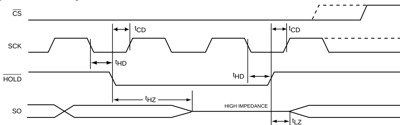
Figure 9. HOLD Timing
