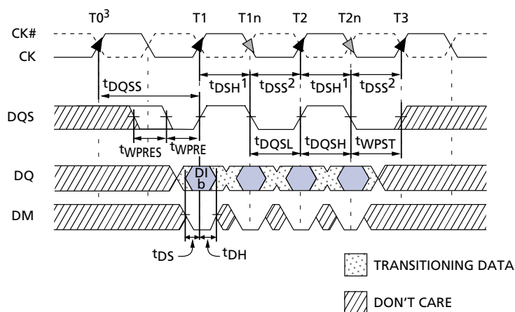
Figure 42: Data Input Timing
