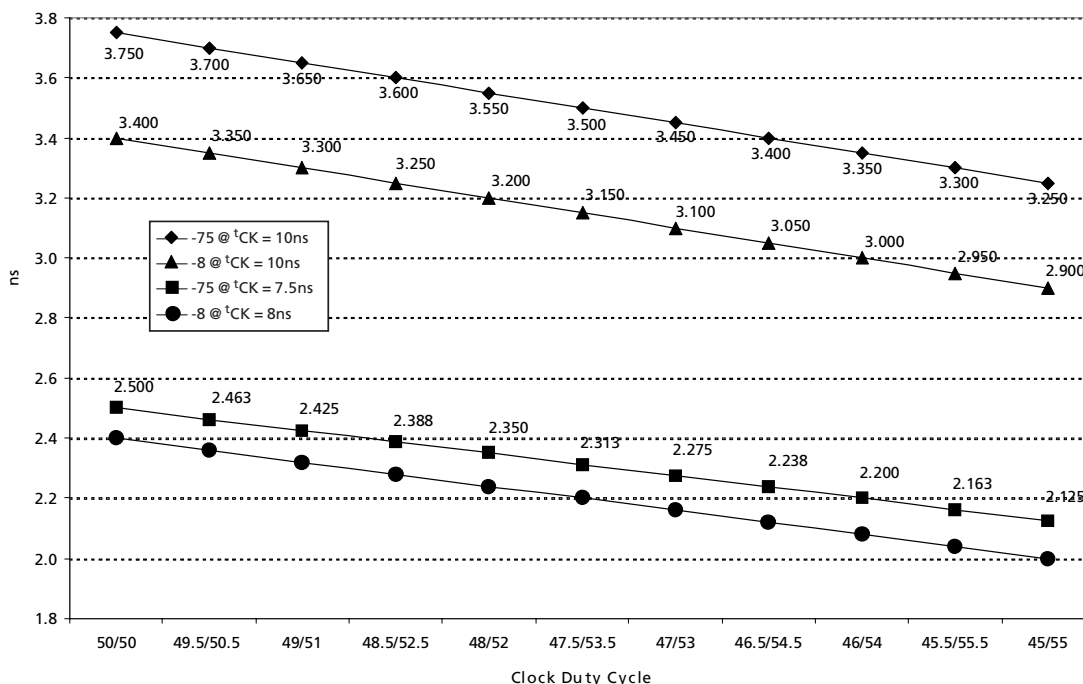
Figure 34: Derating Data Valid Window ( t_{QH} - t_{DQSQ} )
