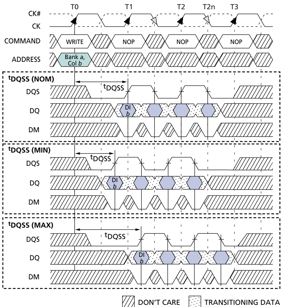
Figure 20: WRITE Burst
