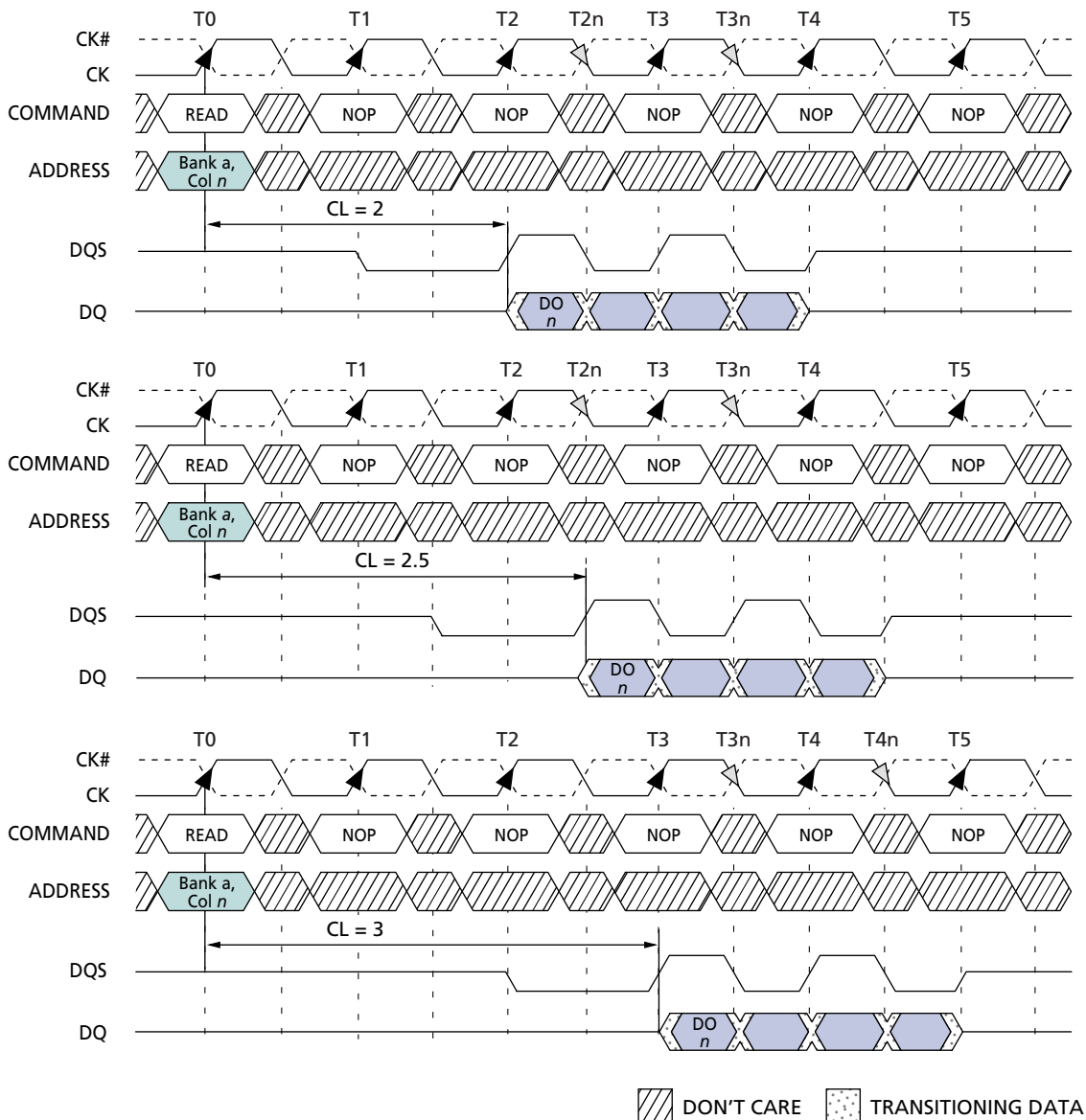
Figure 12: READ Burst
