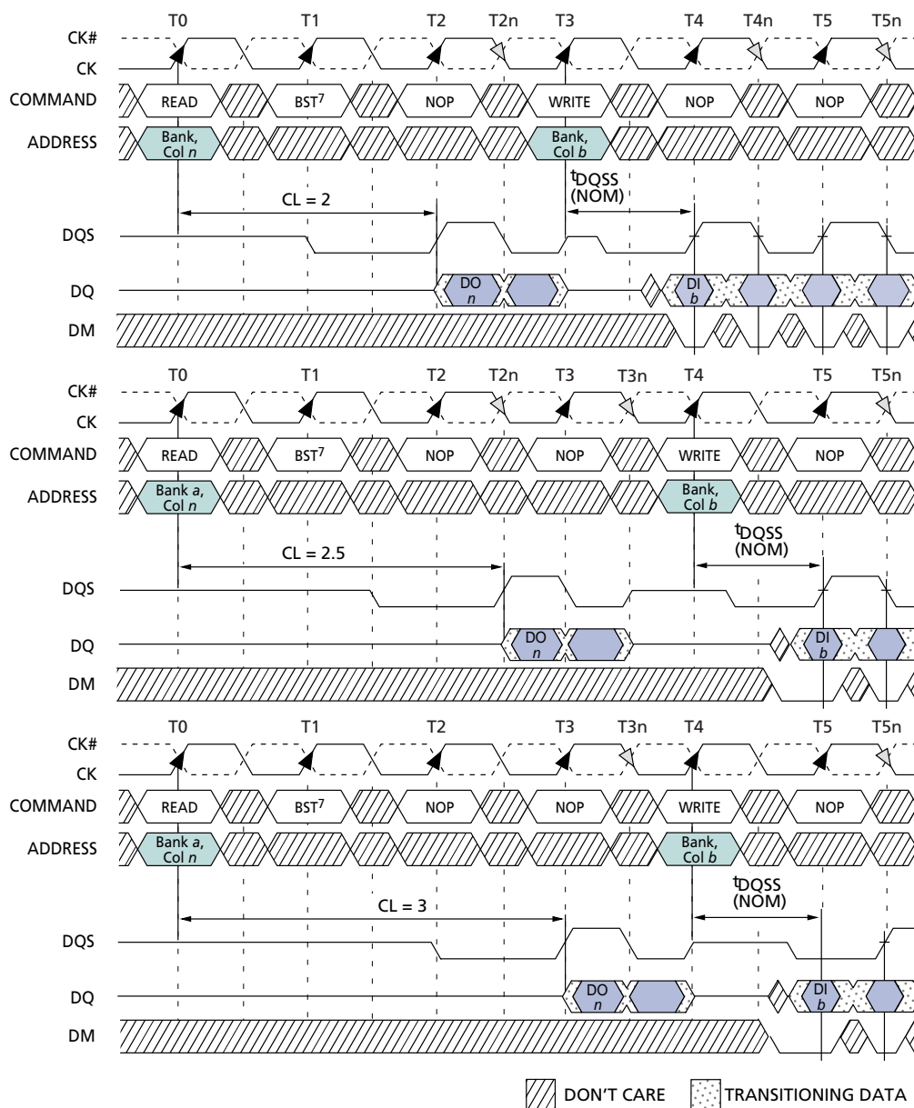
Figure 17: READ to WRITE
