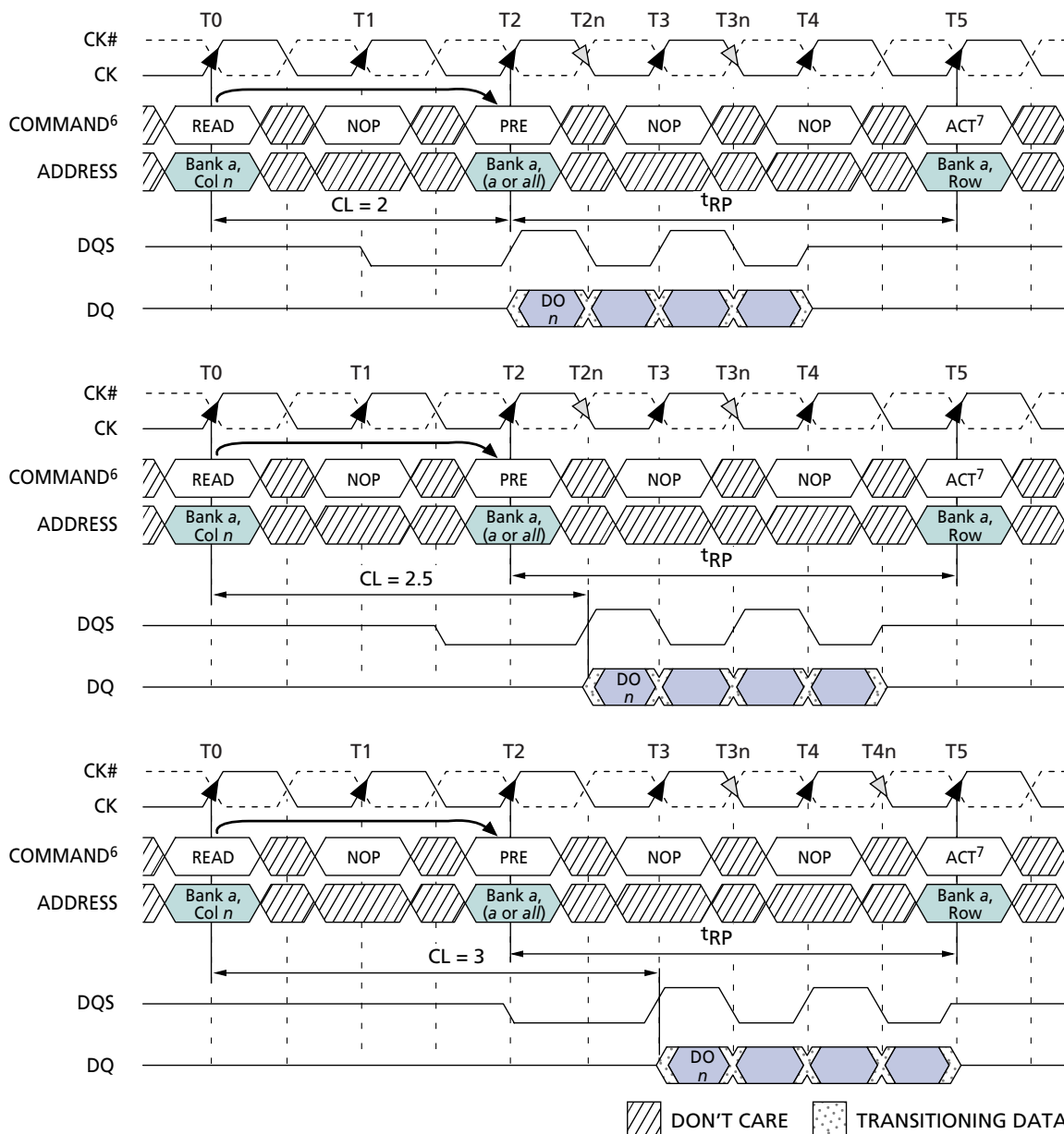
Figure 18: READ to PRECHARGE
