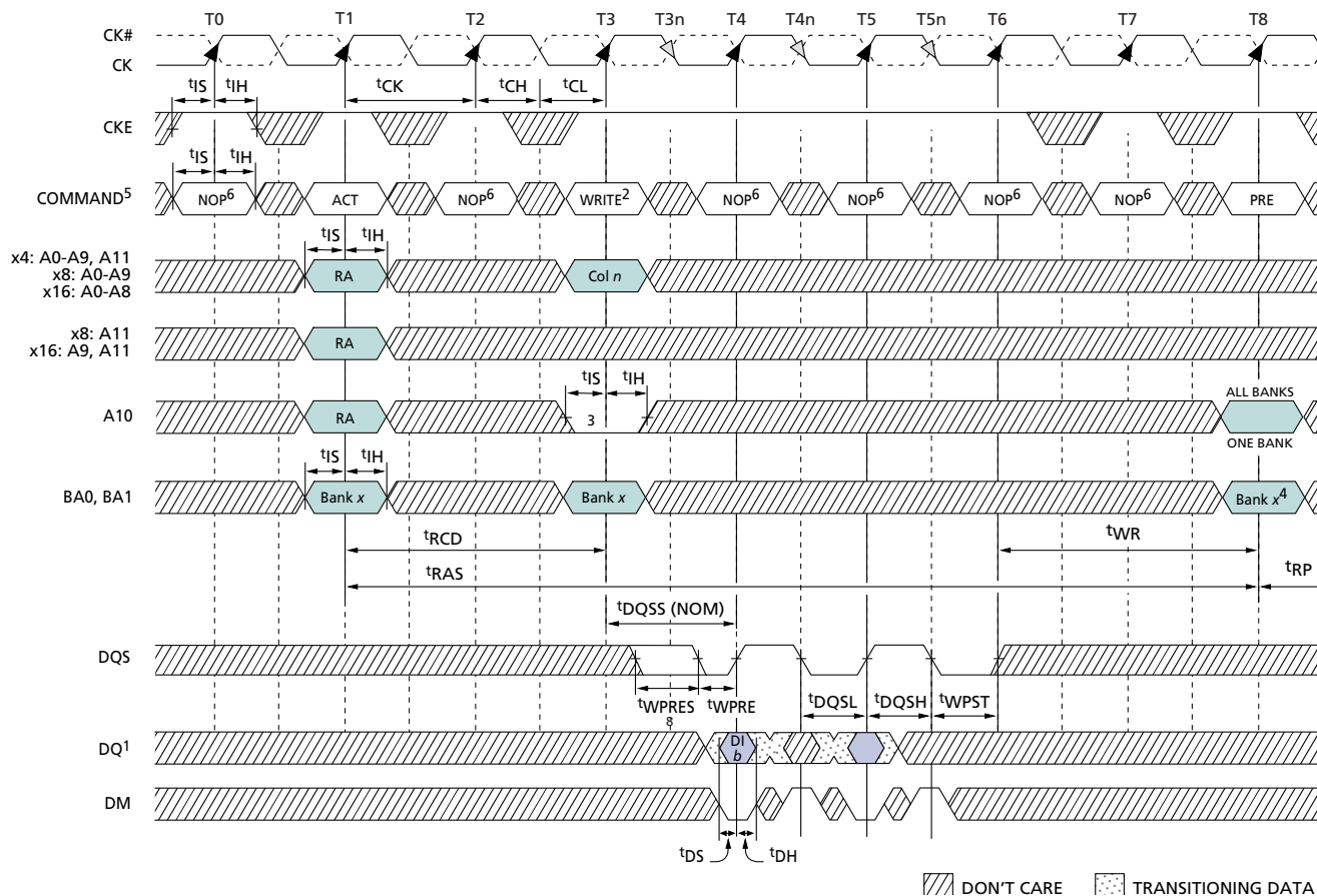
Figure 51: Write - DM Operation
