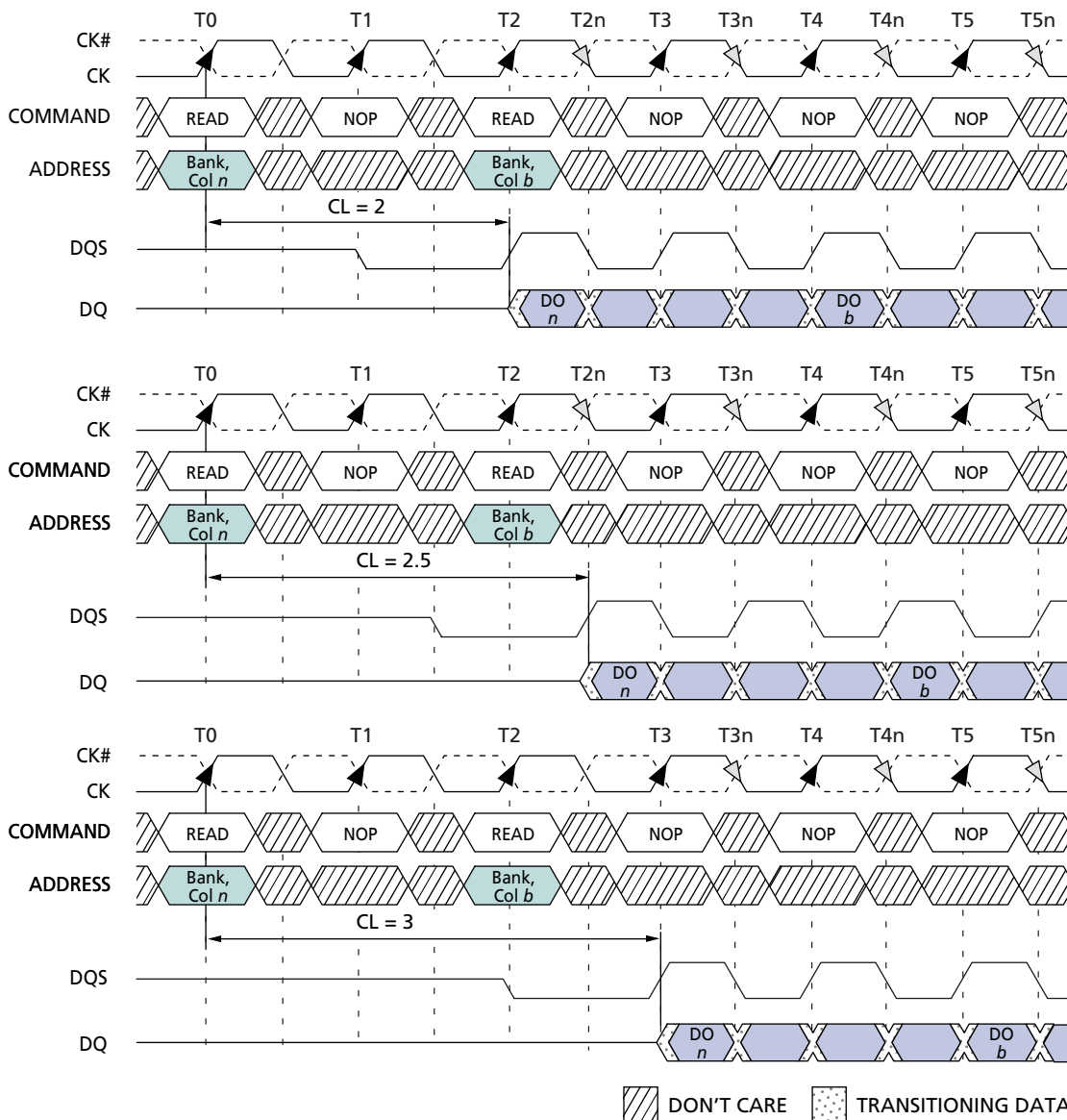
Figure 13: Consecutive READ Bursts
