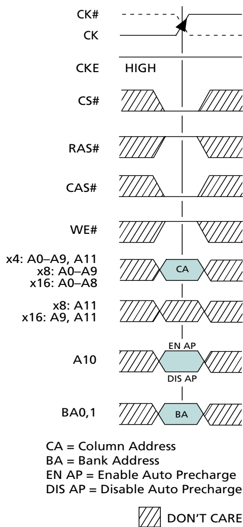
Figure 11: READ Command
