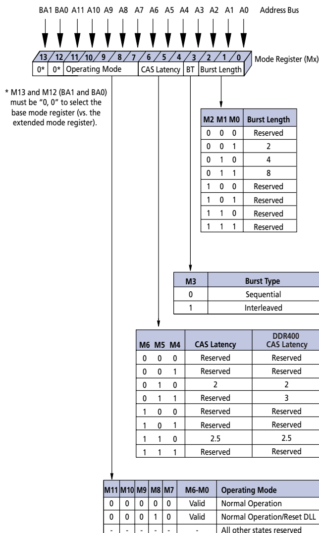
Figure 6: Mode Register Definition
