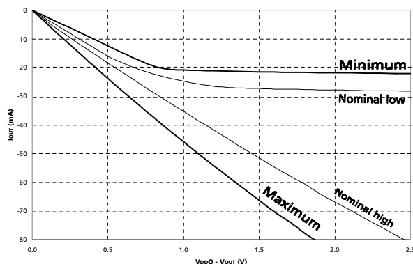
Figure 38: Reduced Drive Pull-Up Characteristics
