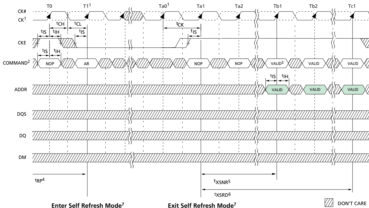
Figure 46: Self Refresh Mode
