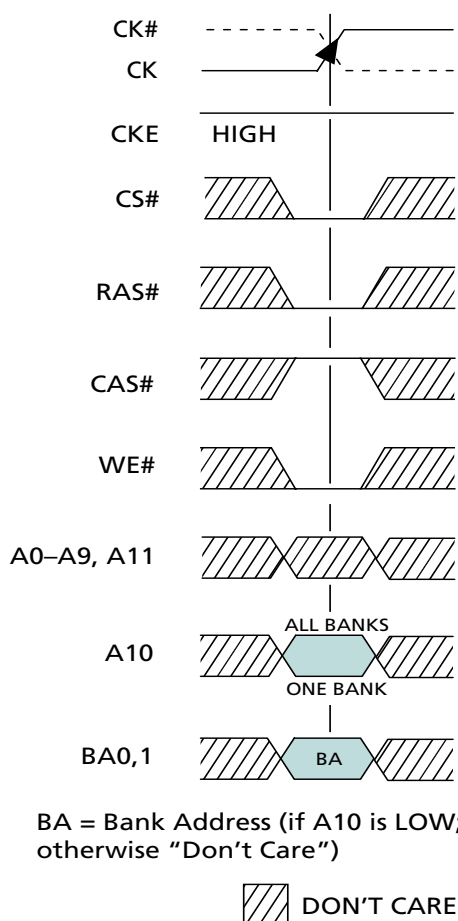
Figure 30: PRECHARGE Command
