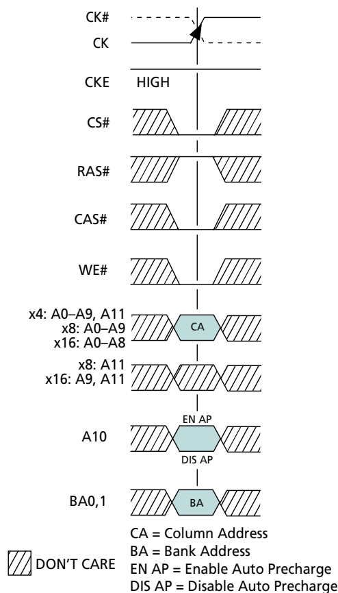
Figure 19: WRITE Command
