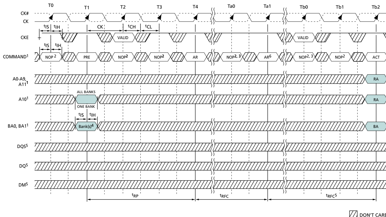
Figure 45: Auto Refresh Mode
