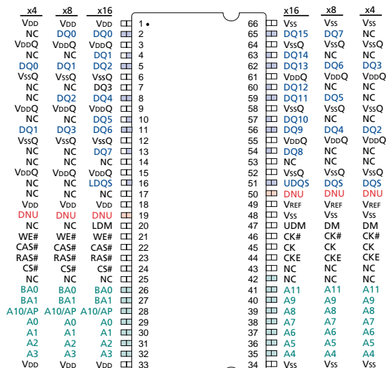
Figure 1: Pin Assignment (Top View) 66-pin TSOP
