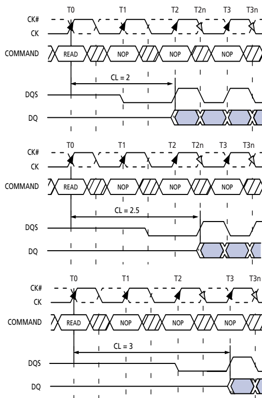
Figure 7: CAS Latency
