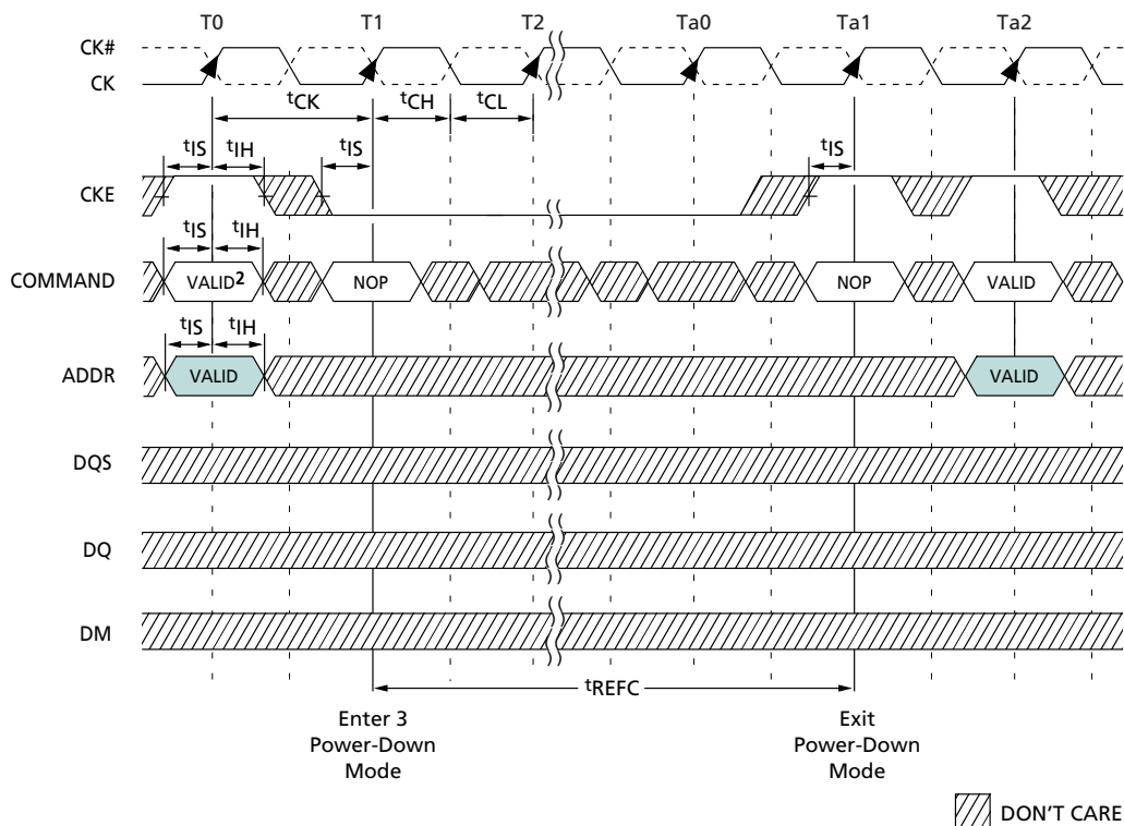
Figure 44: Power-Down Mode
