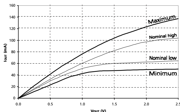
Figure 36: Full Drive Pull-Up Characteristics
