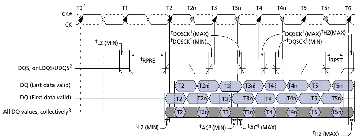
Figure 41: Data Output Timing – t_{AC} and t_{DQSK}
