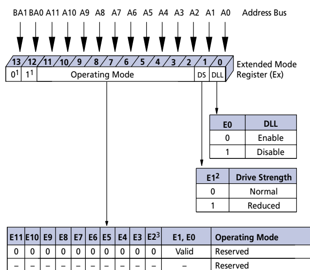
Figure 8: Extended Mode Register Definition
