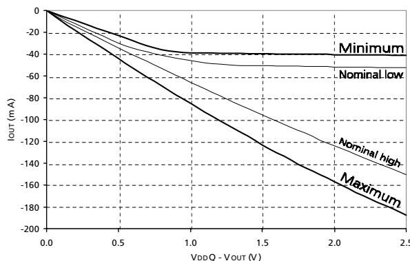
Figure 36: Full Drive Pull-Up Characteristics
