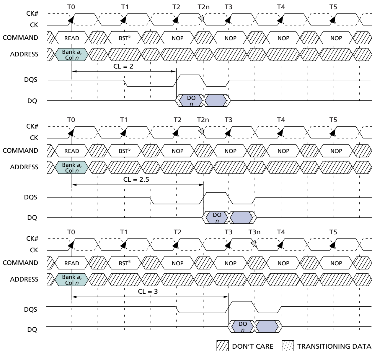
Figure 16: Terminating a READ Burst
