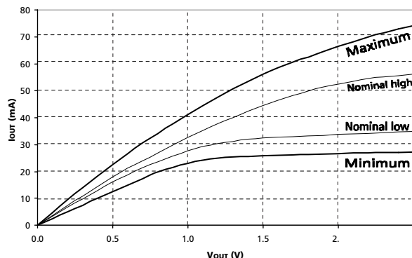
Figure 38: Reduced Drive Pull-Up Characteristics
