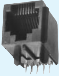
PHJ-8P8C-1-J-5 (shown)
