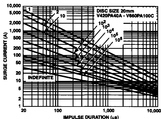
FIGURE 6. SURGE CURRENT RATING CURVES FOR V420PA40A - V660PA100C
