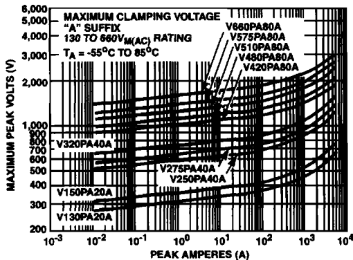
FIGURE 3. CLAMPING VOLTAGE FOR V130PA20A - V660PA100A
