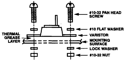
TYPICAL NON-ISOLATED MOUNTING
