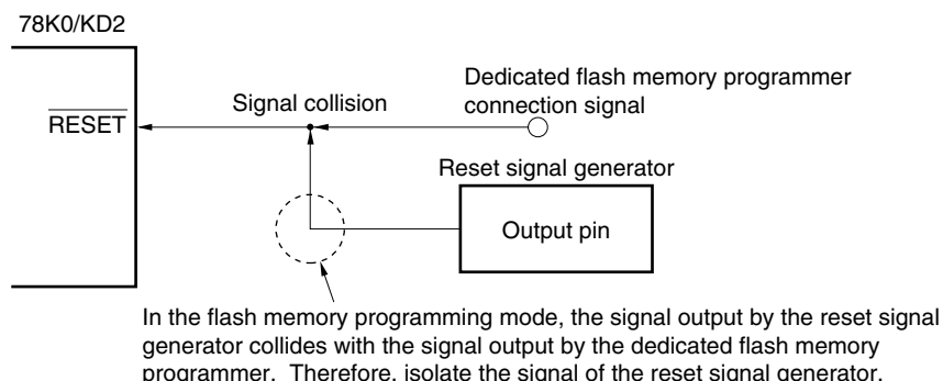
Figure 26-11. Signal Collision ( \overline{\text{RESET}} Pin)
