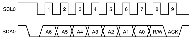
Figure 17-16. \overline{ACK}
