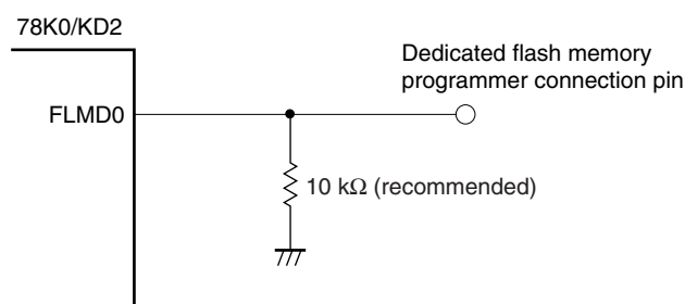
Figure 26-8. FLMD0 Pin Connection Example
