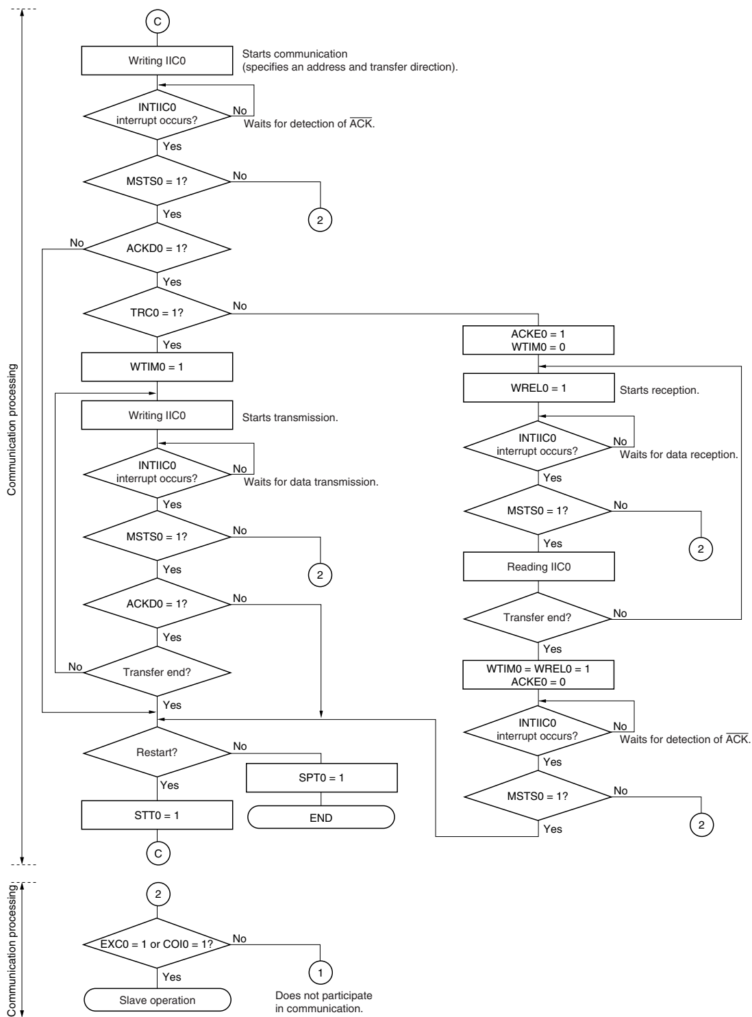
Figure 17-24. Master Operation in Multi-Master System (3/3)
