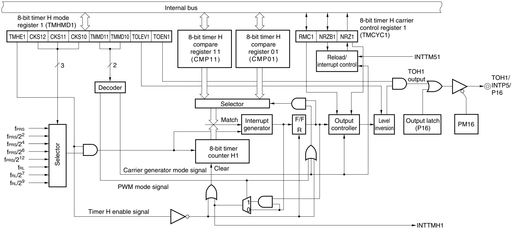
<R> Figure 9-2. Block Diagram of 8-Bit Timer H1
