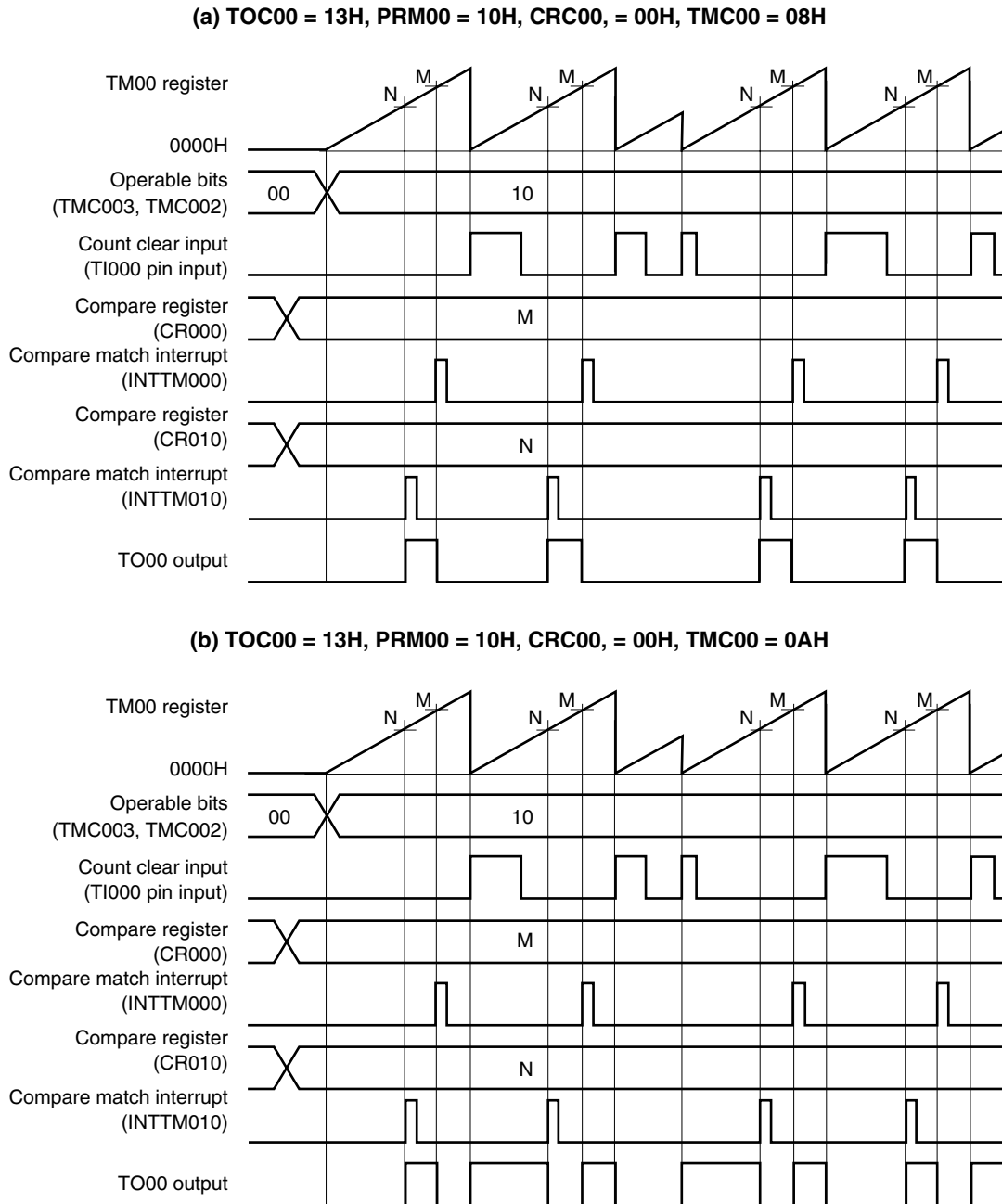
Figure 7-23. Timing Example of Clear & Start Mode Entered by TI000 Pin Valid Edge Input (CR000: Compare Register, CR010: Compare Register)
