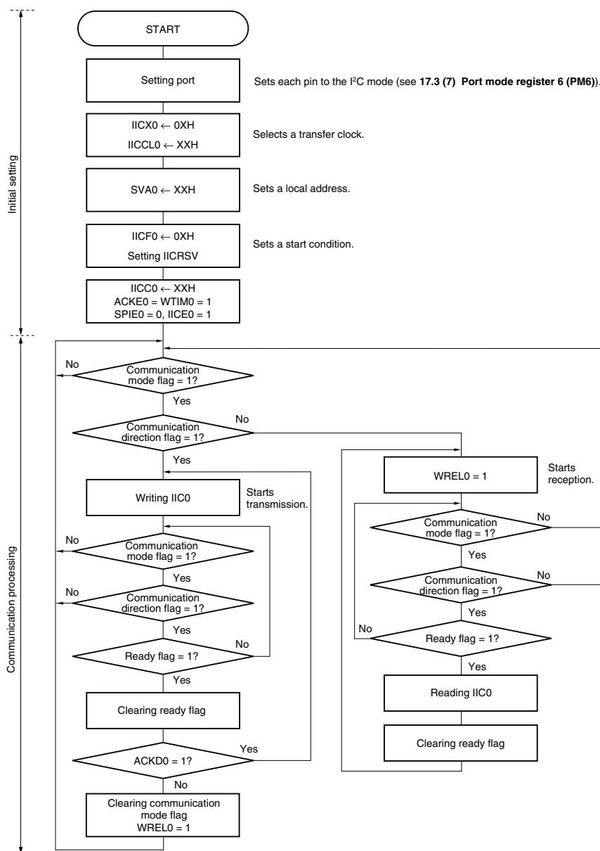
Figure 17-25. Slave Operation Flowchart (1)
