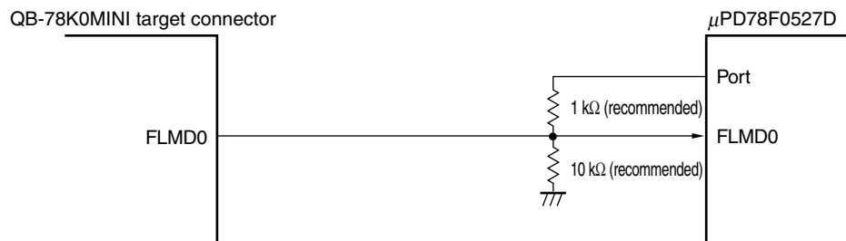
Figure 27-3. Connection of FLMD0 Pin for Self Programming by Means of On-Chip Debugging
