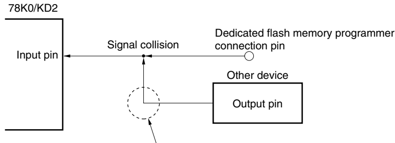
Figure 26-9. Signal Collision (Input Pin of Serial Interface)
