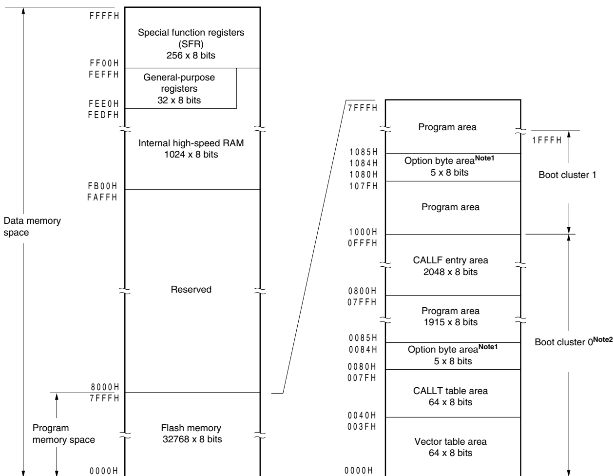
Figure 3-3. Memory Map ( \mu PD78F0523)
