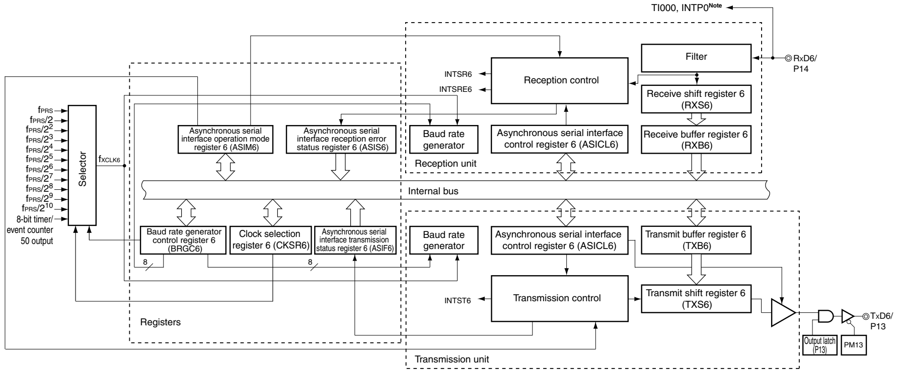
<R>Figure 15-4. Block Diagram of Serial Interface UART6
