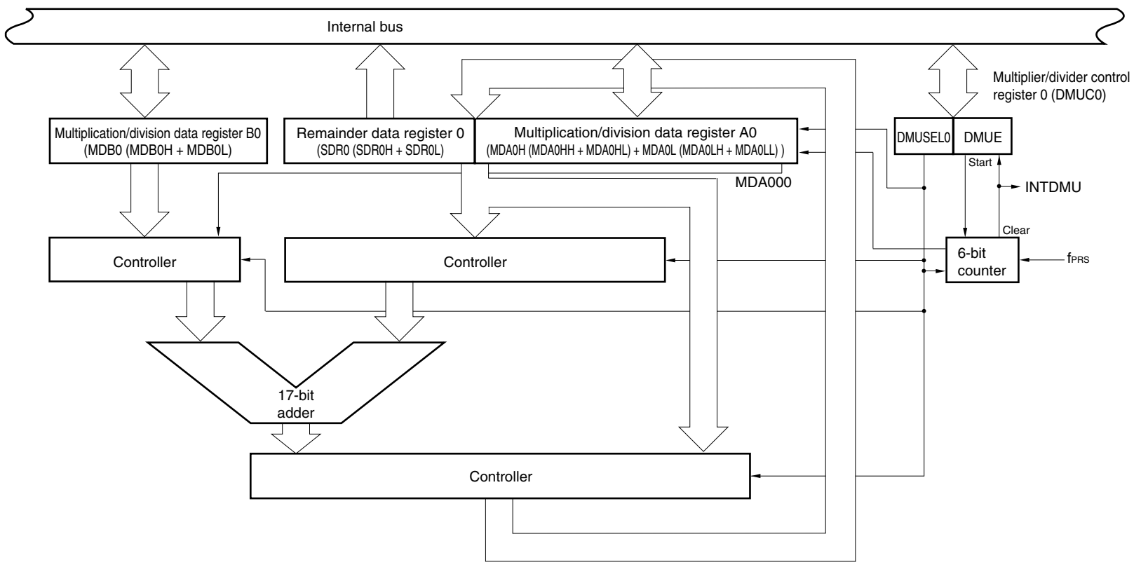
Figure 18-1. Block Diagram of Multiplier/Divider
