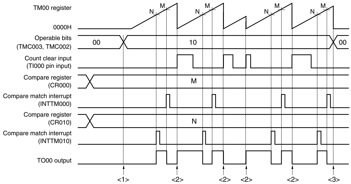
<R> Figure 7-31. Example of Software Processing in Clear & Start Mode Entered by TI000 Pin Valid Edge Input
