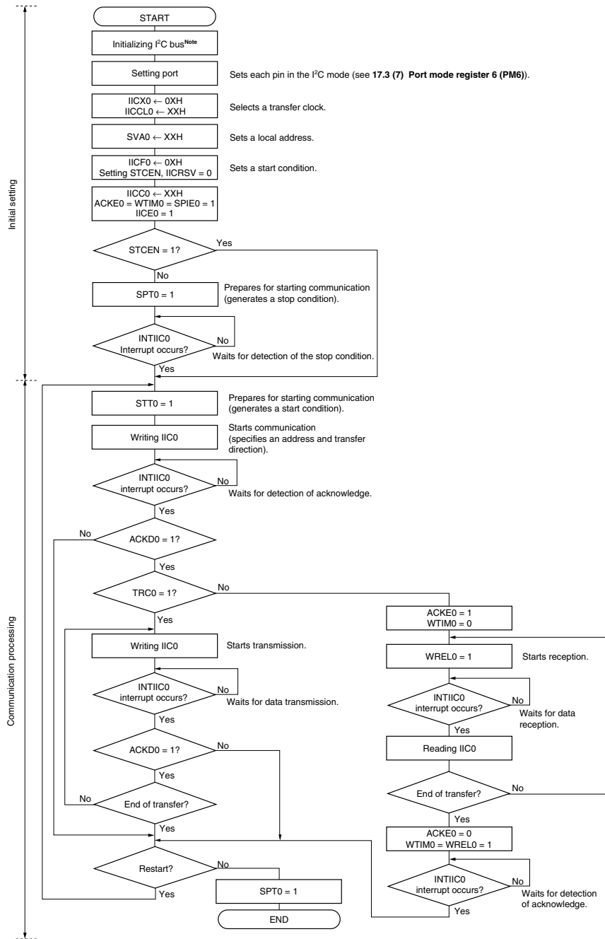
Figure 17-23. Master Operation in Single-Master System
