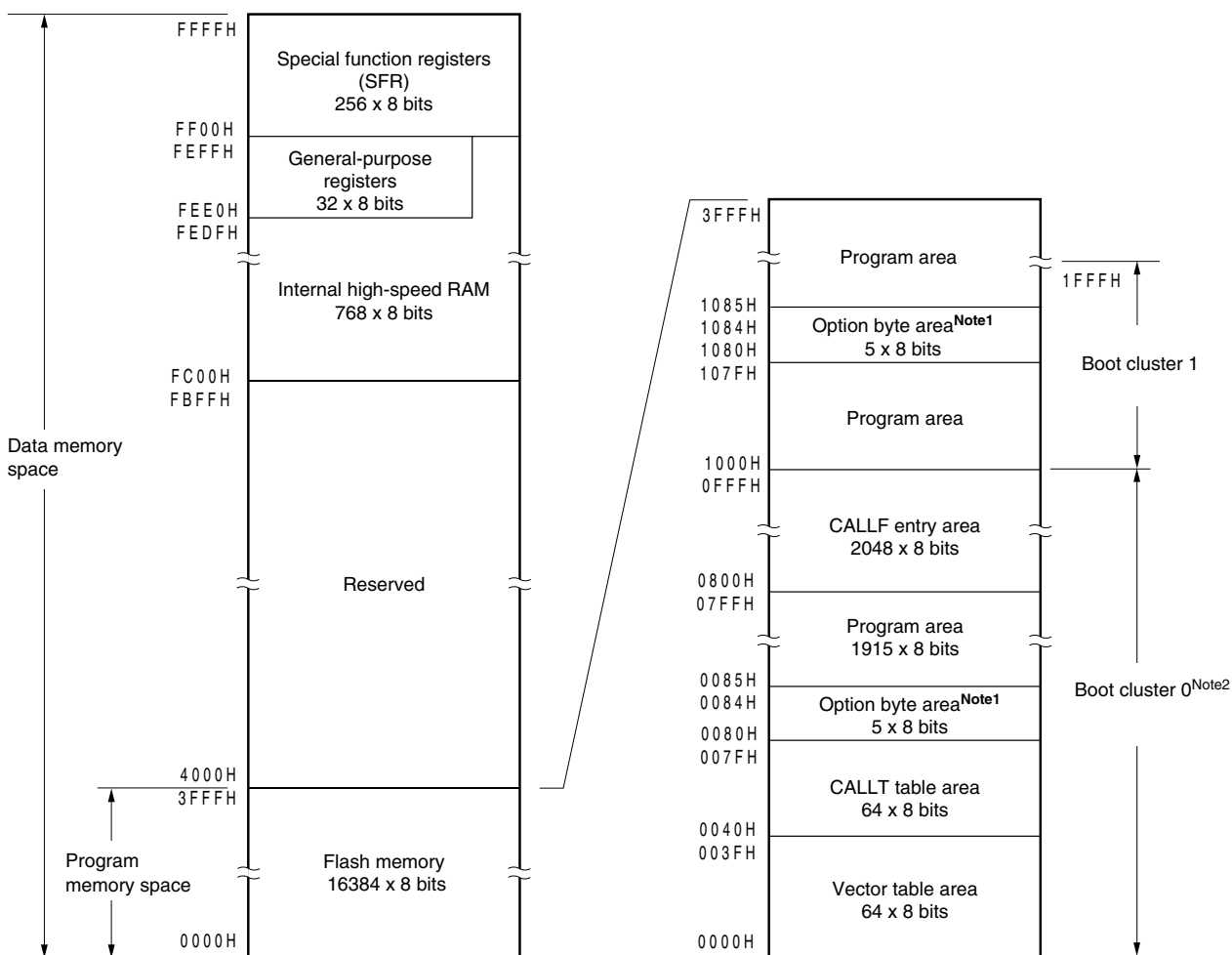
Figure 3-1. Memory Map ( \mu PD78F0521)
