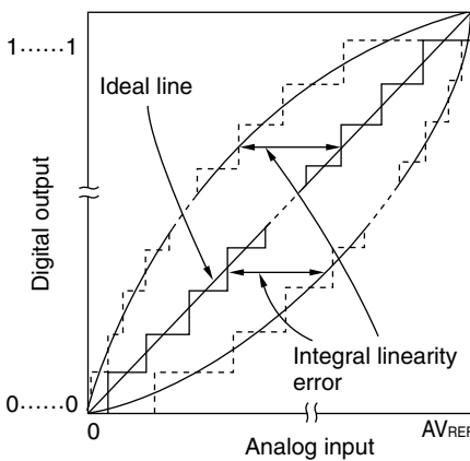
Figure 13-18. Integral Linearity Error
