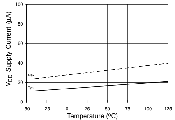
Figure 19A. V DD Supply Current vs. Temperature
