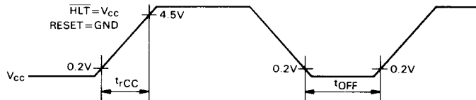
Figure 18 Power Supply Timing for Built-in Reset Circuit
