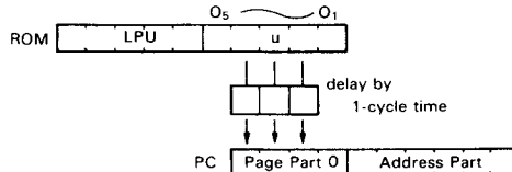
Figure 7 LPU Operation
