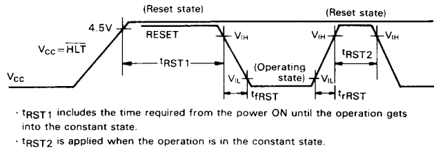
Figure 17 RESET Timing
