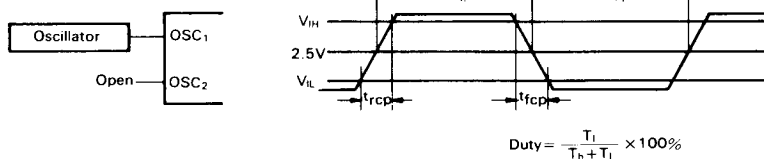
Figure 20 Clock Operation Mode
