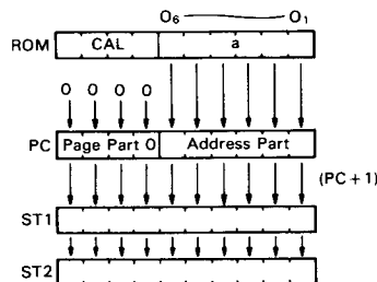
Figure 9 Subroutine Jump Stacking Order
