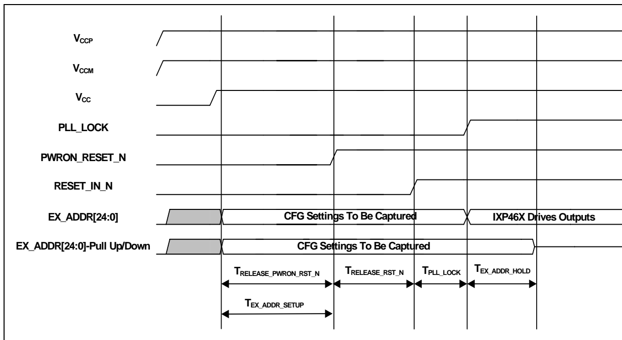
Figure 49. Reset Timings
