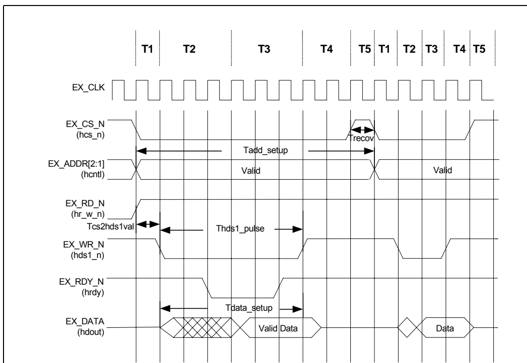
Figure 39. HPI*-16 Multiplexed Read Mode
