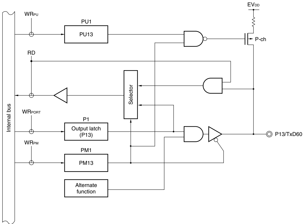
Figure 5-6. Block Diagram of P13
