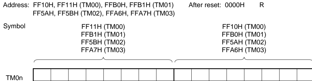
Figure 7-7. Format of 16-Bit Timer Counter 0n (TM0n)
