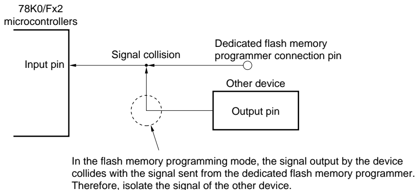
Figure 24-15. Signal Collision (Input Pin of Serial Interface)
