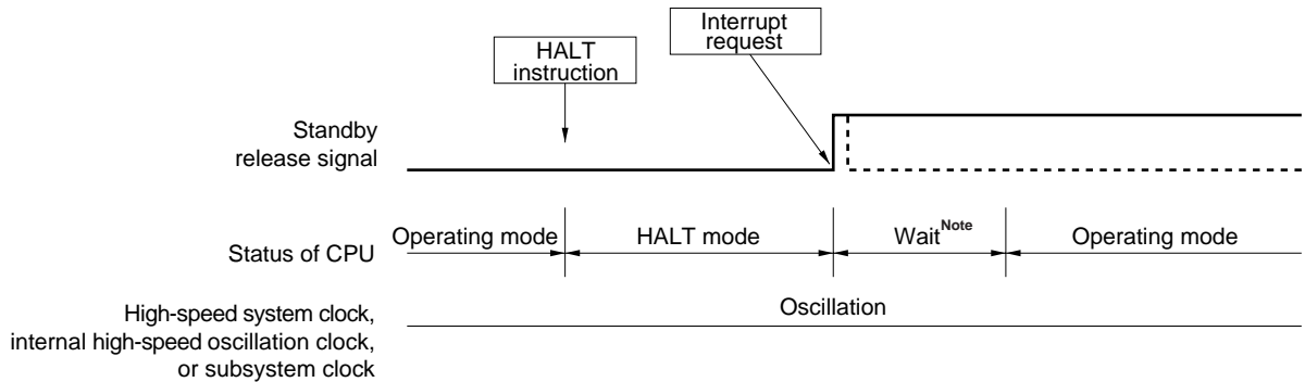
Figure 18-3. HALT Mode Release by Interrupt Request Generation
