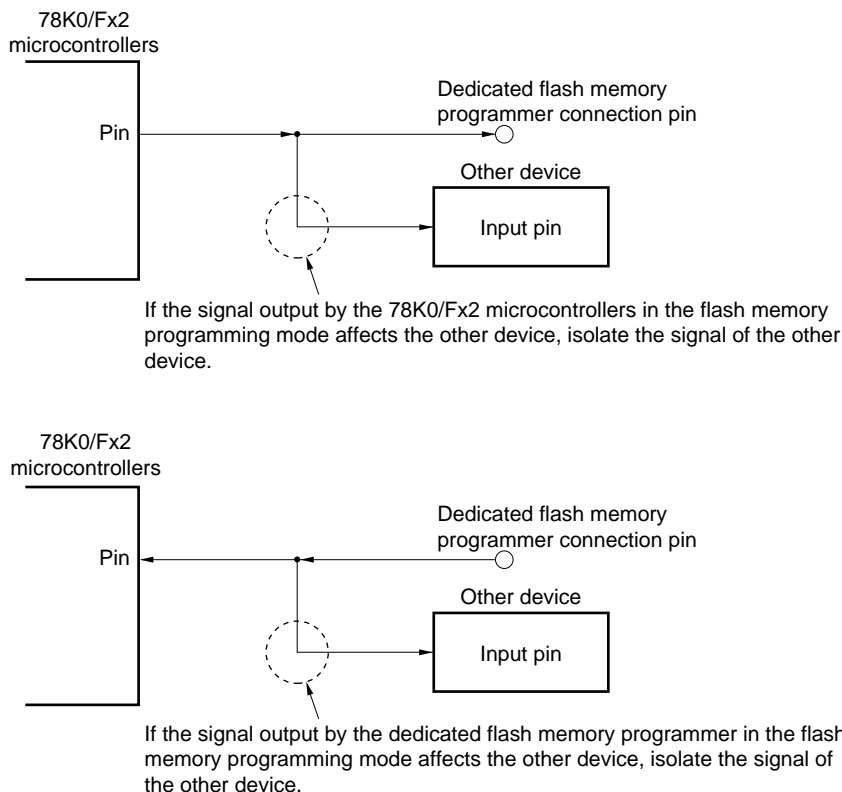
Figure 24-16. Malfunction of Other Device
