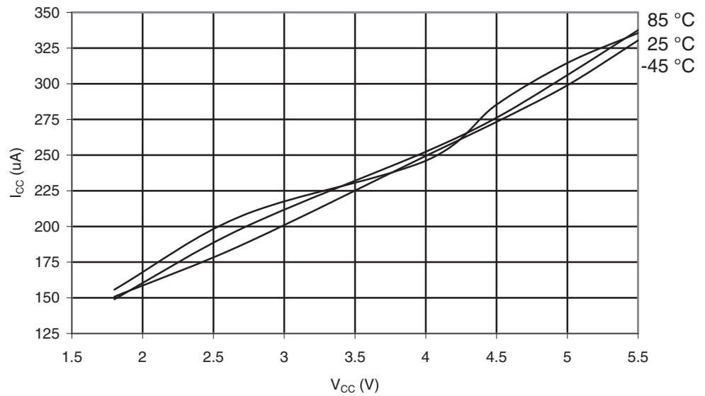
Figure 30-55. ATmega169A: Active Supply Current with ADC at 1MHz vs. V_{CC}
