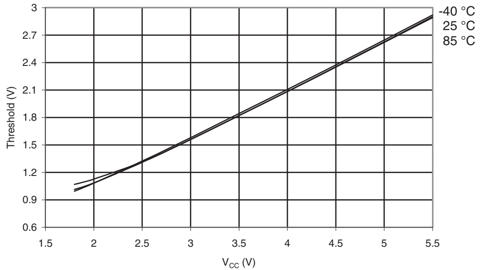
Figure 30-278. ATmega3290A: I/O Pin Input Threshold Voltage vs. V_{CC} ( V_{IH} , I/O Pin Read as "1")
