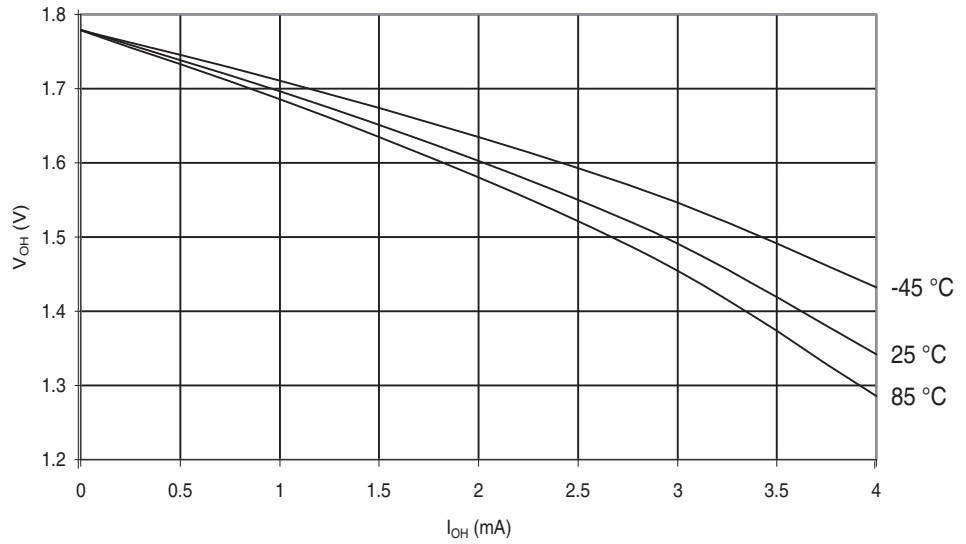
Figure 30-390. ATmega649A: I/O Pin Output Voltage vs. Source Current, Port B ( V_{CC} = 5V )
