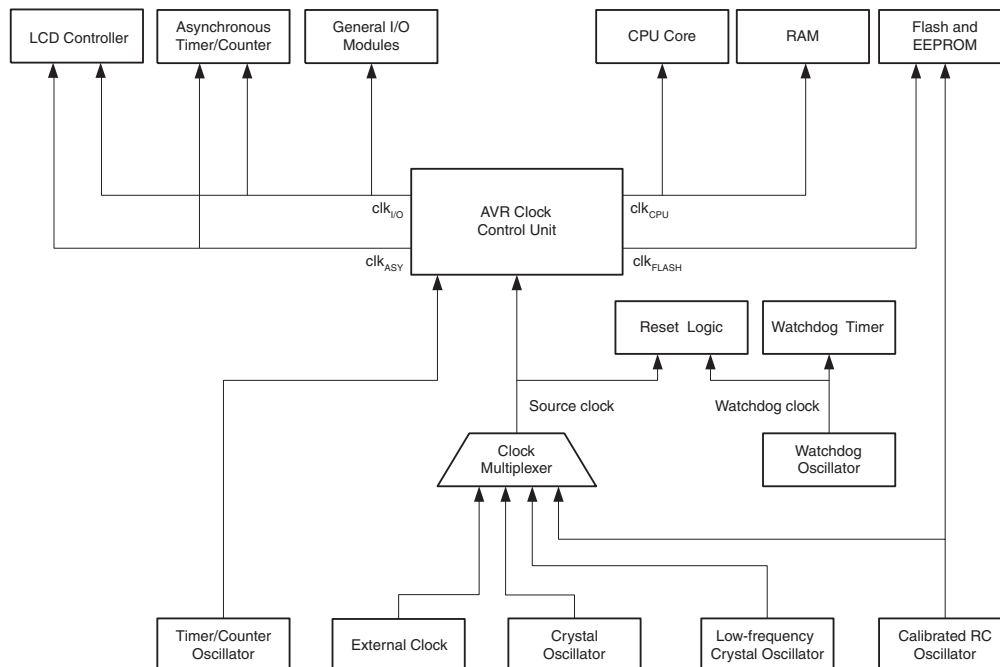
Figure 9-1. Clock Distribution
