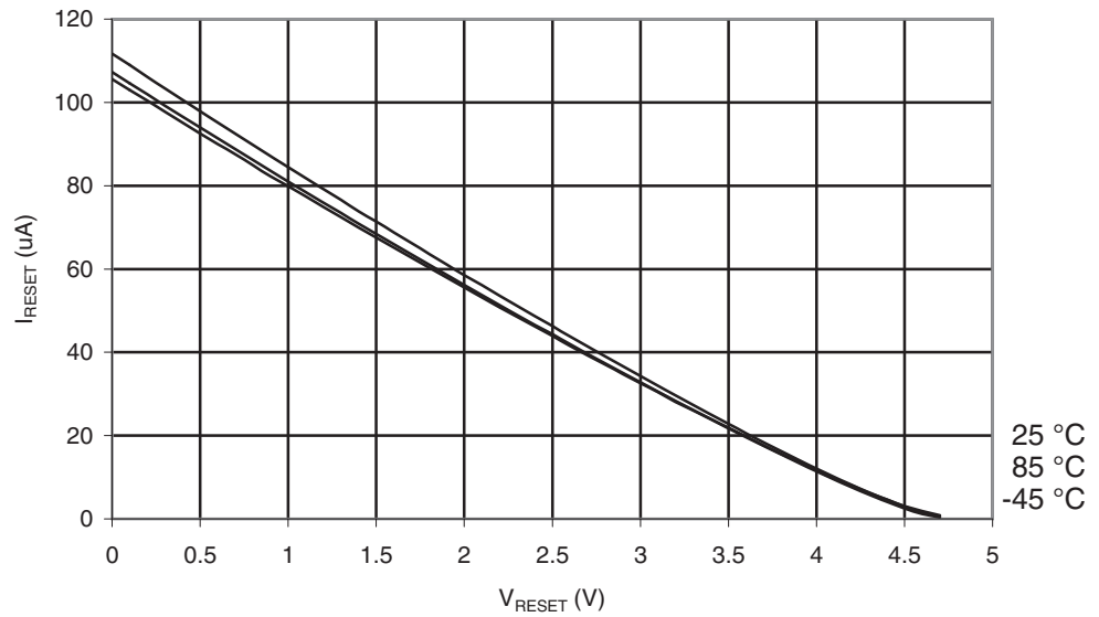
Figure 30-81. ATmega169PA: Reset Pull-up Resistor Current vs. Reset Pin Voltage ( V_{CC} = 5V )
