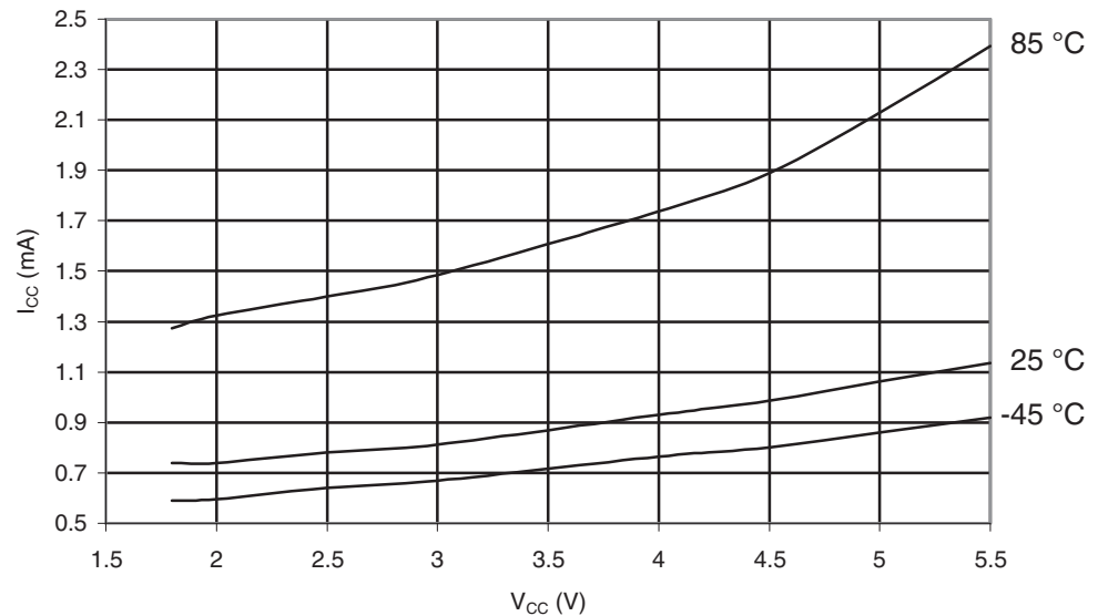
Figure 30-500. ATmega6490A: Power-save Supply Current vs. V_{CC} (Watchdog Timer Disabled and 32kHz Crystal Oscillator Running)
