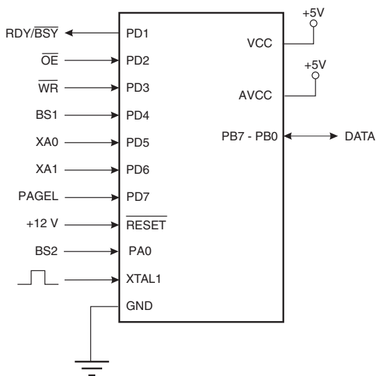
Figure 28-1. Parallel Programming
