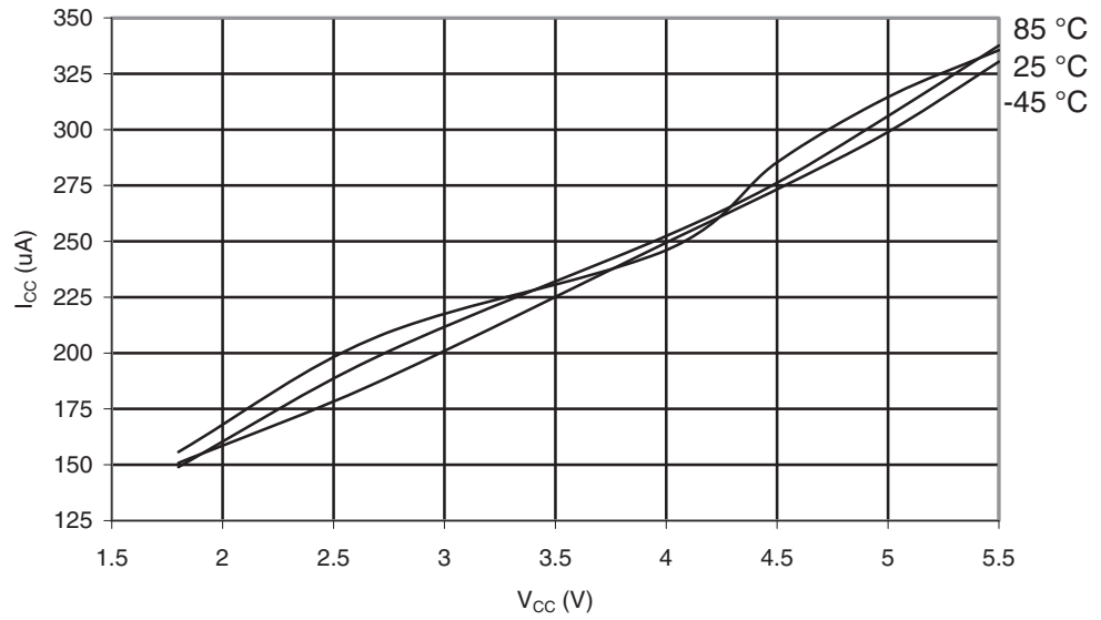
Figure 30-117. ATmega169PA: Active Supply Current with ADC at 1MHz vs. V_{CC}
