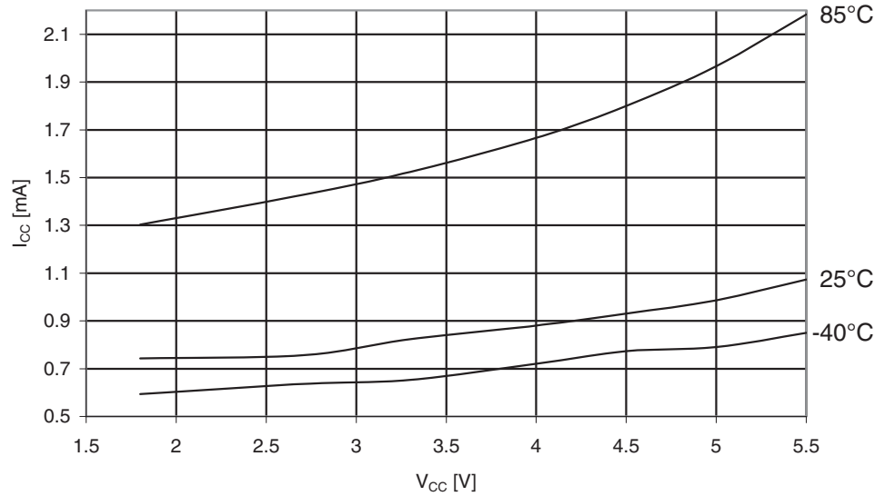
Figure 30-138. ATmega329A Standby Supply Current vs. V_{CC} (32kHz Watch Crystal, Watchdog Timer Disabled)
