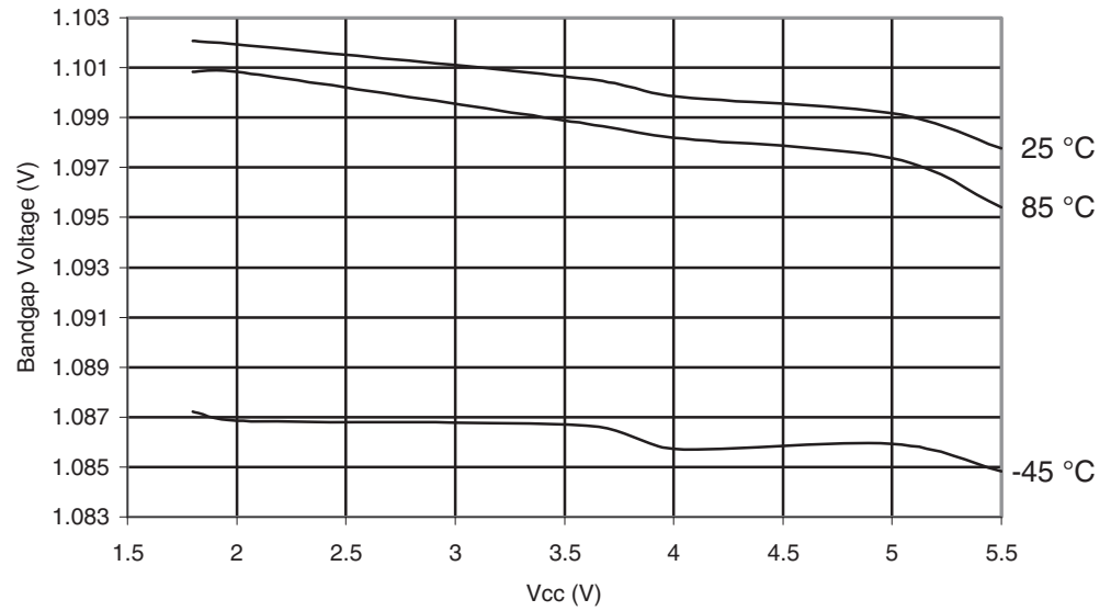
Figure 30-469. ATmega649P: Bandgap Voltage vs. V CC
