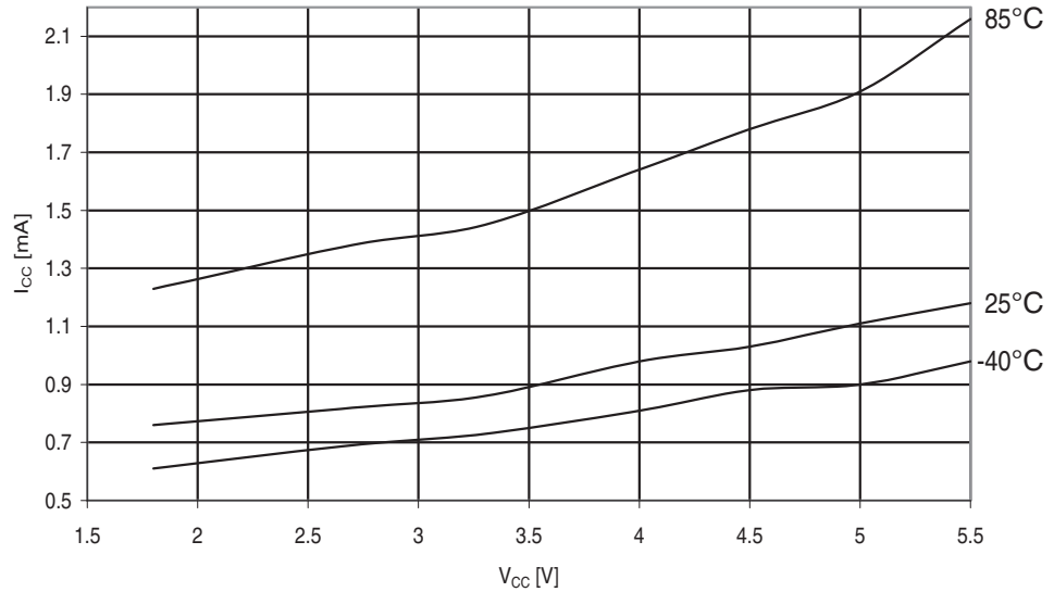
Figure 30-257. ATmega3290A: Power-save Supply Current vs. V_{CC} (Watchdog Timer Disabled and 32kHz Crystal Oscillator Running)
