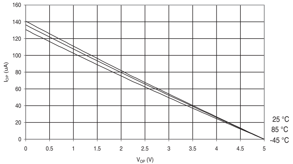
Figure 30-503. ATmega6490A: I/O Pin Pull-up Resistor Current vs. Input Voltage ( V_{CC} = 5V )
