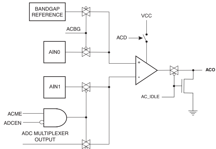
Figure 26-6. Analog Comparator
