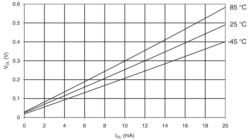
Figure 30-93. ATmega169PA: I/O Pin Output Voltage vs. Sink Current, Port B ( V_{CC} = 5V )
