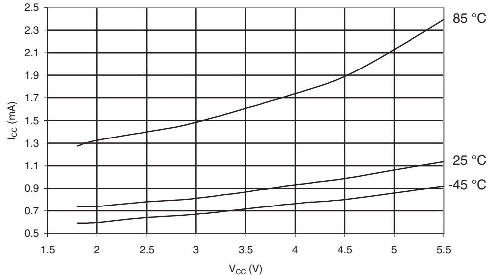
Figure 30-561. ATmega6490P: Power-save Supply Current vs. V_{CC} (Watchdog Timer Disabled and 32kHz Crystal Oscillator Running)
