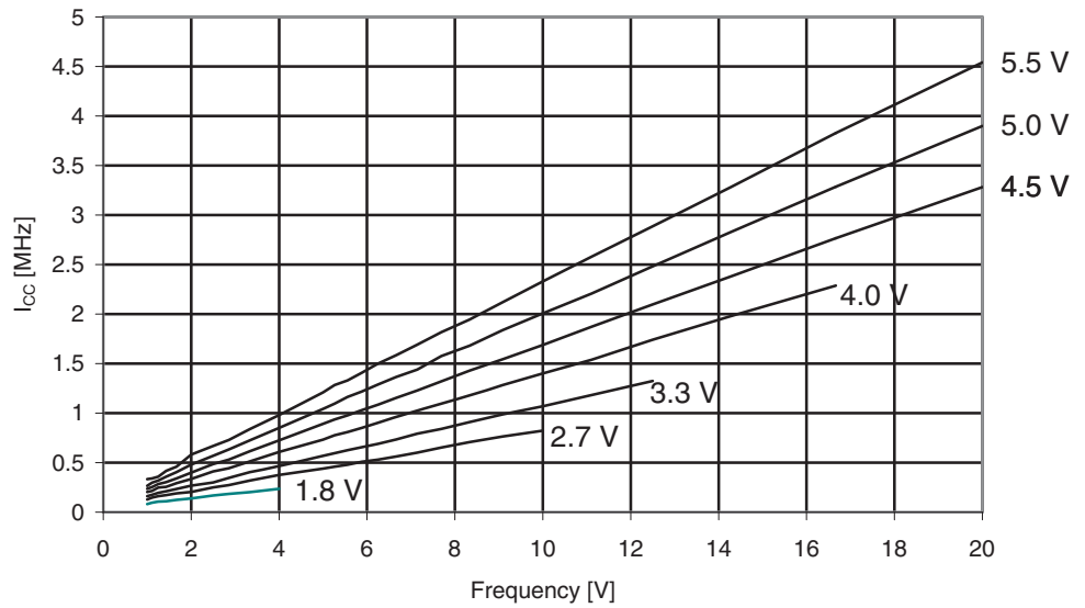
Figure 30-131. ATmega329A: Idle Supply Current vs. Frequency (1 - 20MHz)
