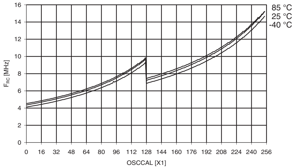
Figure 30-233. ATmega329PA: Calibrated 8MHz RC Oscillator Frequency vs. Oscscal Value
