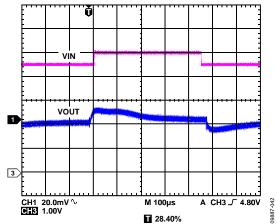
Figure 38. LDO Response to Line Transient, Input Voltage from 4.5 V to 5.5 V, V_{OUT3} = 2.8V
