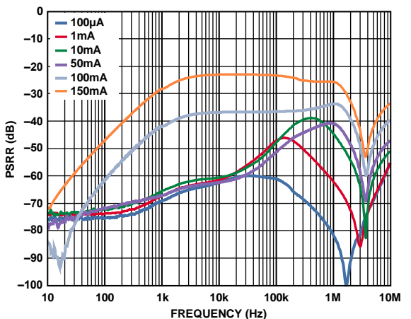
Figure 41. LDO PSRR Across Output Load, V_{IN3} = 3.3V, V_{OUT3} = 2.8V
