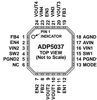
Figure 2. Pin Configuration—View from the Top of the Die
