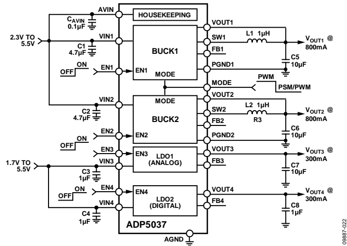
Figure 52. ADP5037 Fixed Output Voltages with Enable Pins
