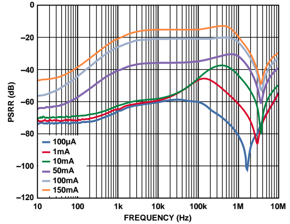
Figure 42. LDO PSRR Across Output Load, V_{IN3} = 3.3V, V_{OUT3} = 3.0V
