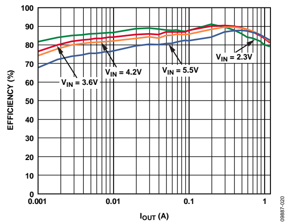
Figure 11. BUCK2 Efficiency vs. Load Current, Across Input Voltage, V_{out2} = 1.8V , Auto Mode
