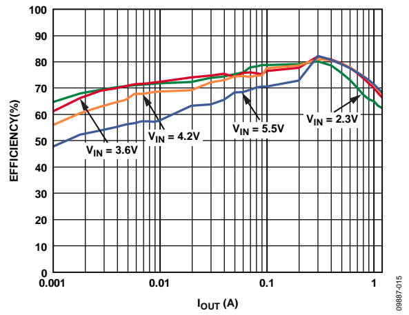
Figure 13. BUCK1 Efficiency vs. Load Current, Across Input Voltage, V_{out1} = 0.8V , Auto Mode
