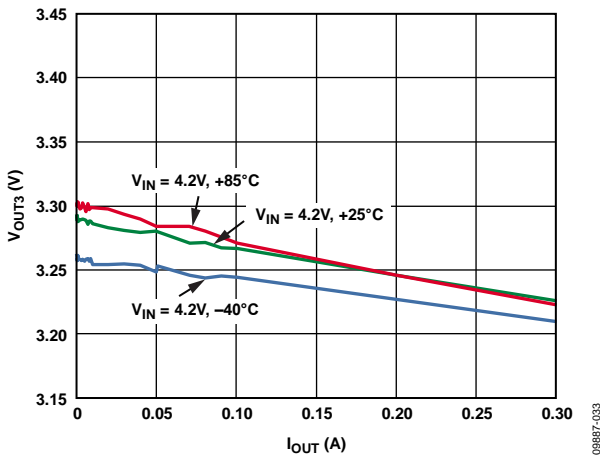
Figure 34. LDO Load Regulation Across Temperature, V_{IN3} = 3.3V , V_{OUT3} = 2.8V
