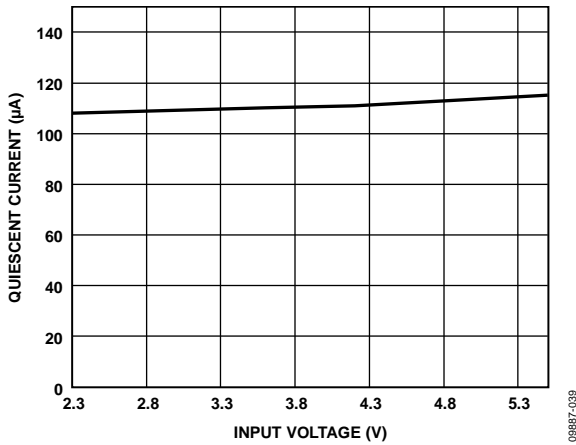
Figure 3. System Standby Current vs. Input Voltage, V_{OUT1} = 3.3\text{ V} , V_{OUT2} = 1.8\text{ V} , V_{OUT3} = 1.2\text{ V} , V_{OUT4} = 3.3\text{ V} , All Channels Unloaded
