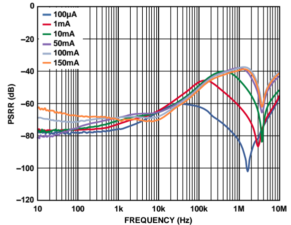
Figure 43. LDO PSRR Across Output Load, V_{IN3} = 5.0V, V_{OUT3} = 2.8V
