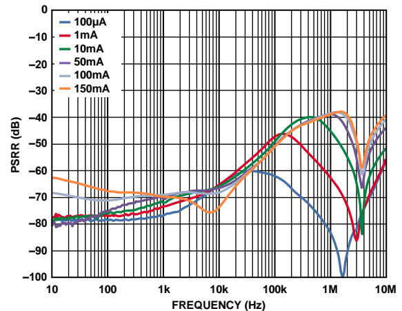
Figure 44. LDO PSRR Across Output Load, V_{IN3} = 5.0V, V_{OUT3} = 3.0V
