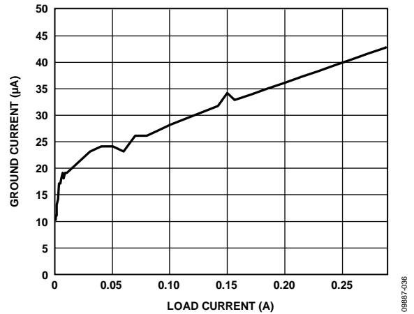
Figure 36. LDO Ground Current vs. Output Load, V_{IN3} = 3.3V , V_{OUT3} = 2.8V
