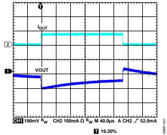
Figure 37. LDO Response to Load Transient, I_{OUT3} from 1 mA to 80 mA, V_{OUT3} = 2.8V
