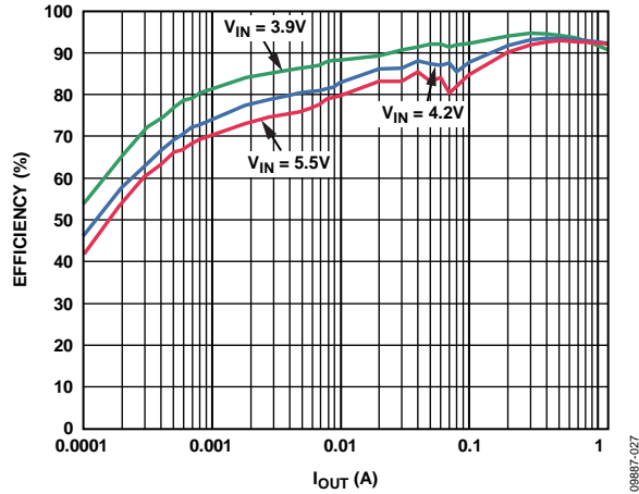
Figure 9. BUCK1 Efficiency vs. Load Current, Across Input Voltage, V_{out1} = 3.3V , Auto Mode
