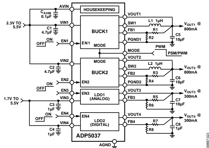
Figure 53. ADP5037 Adjustable Output Voltages with Enable Pins
