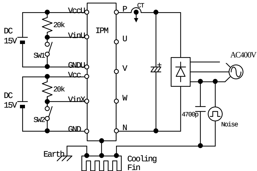
Figure 5. Noise Test Circuit
