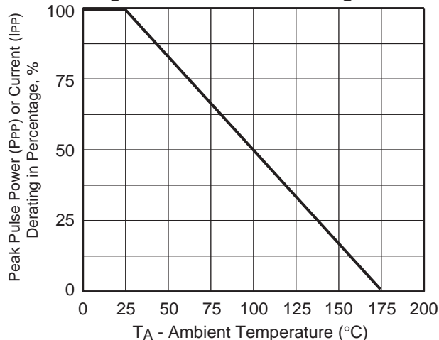
Fig. 2 - Pulse Power Derating Curve
